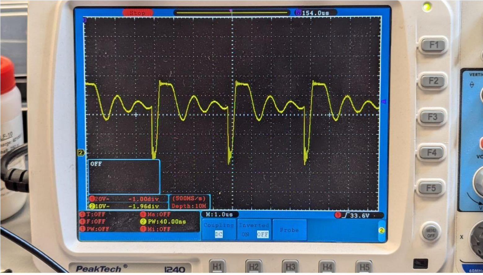
switching node zoom, two waveforms alternating each other:
