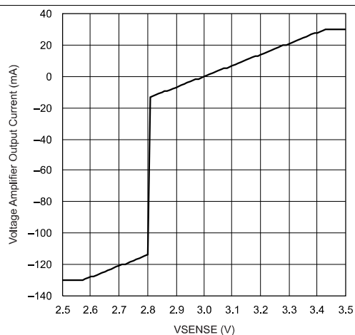
Figure 10. Voltage Amplifier Transfer Function vs V_{VSENSE}
