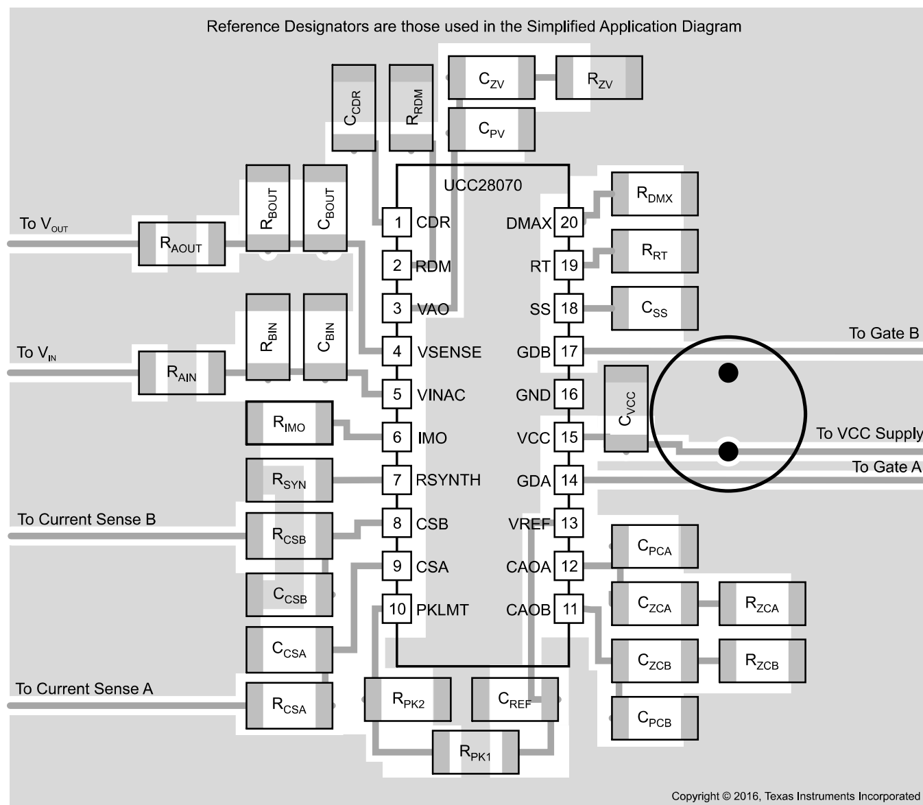
Figure 33. Layout Diagram
