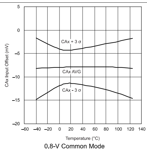
Figure 12. CAX Input Offset Voltage vs Junction Temperature
