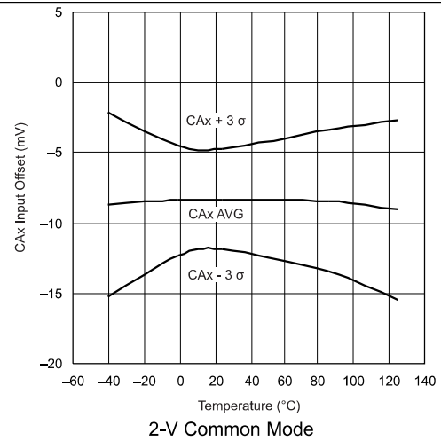
Figure 14. CAx Input Offset Voltage vs Junction Temperature
