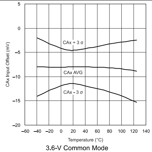
Figure 16. CAx Input Offset Voltage vs Junction Temperature
