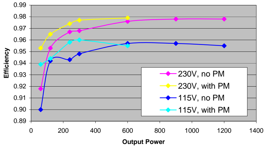
PFC Efficiency without and with Light-load Phase Management
