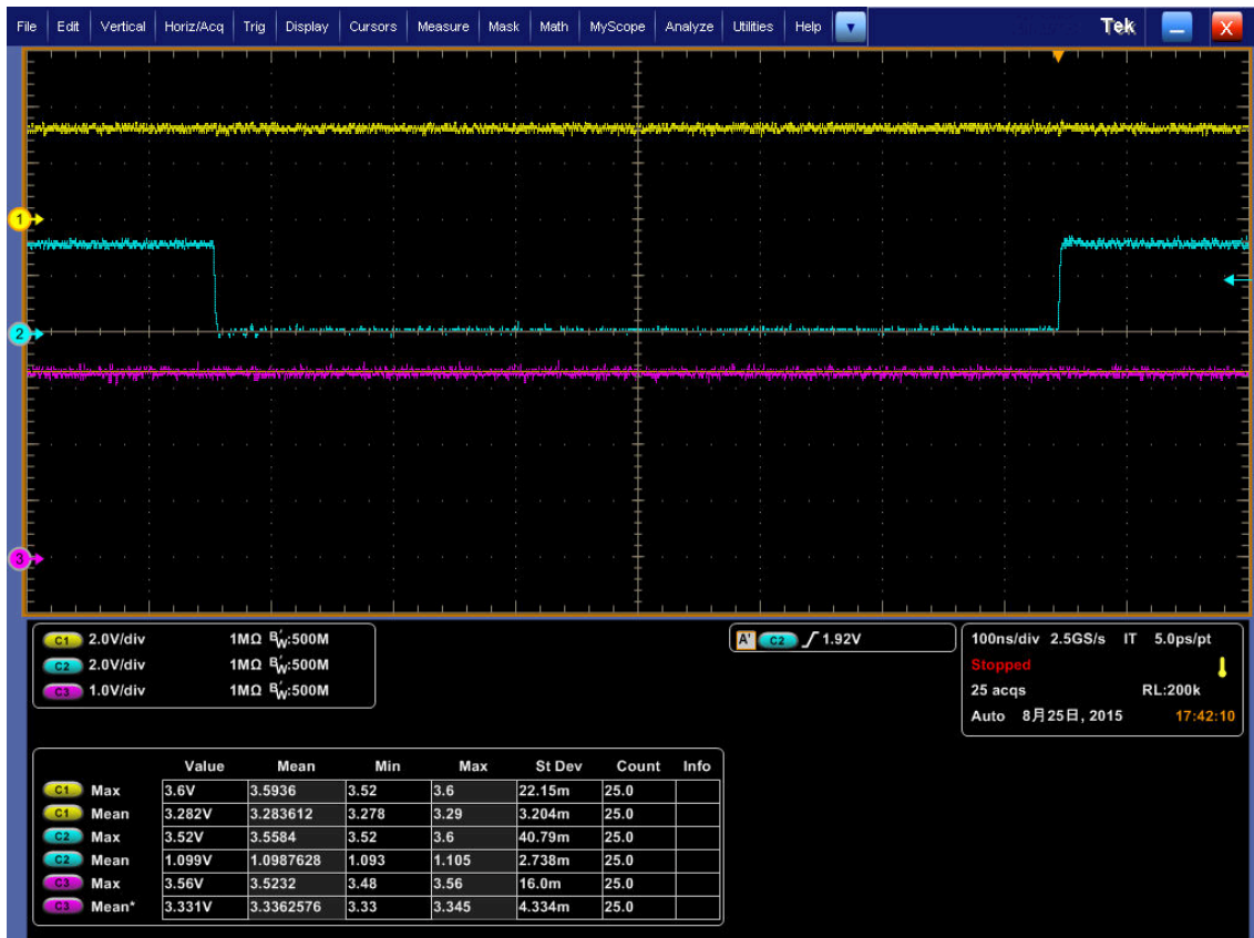
Fig. 7. OUT1 (CH1) , OUT2 (CH2) , REF 端子 (CH3) 電圧波形 (横軸 100nsec./div.)
