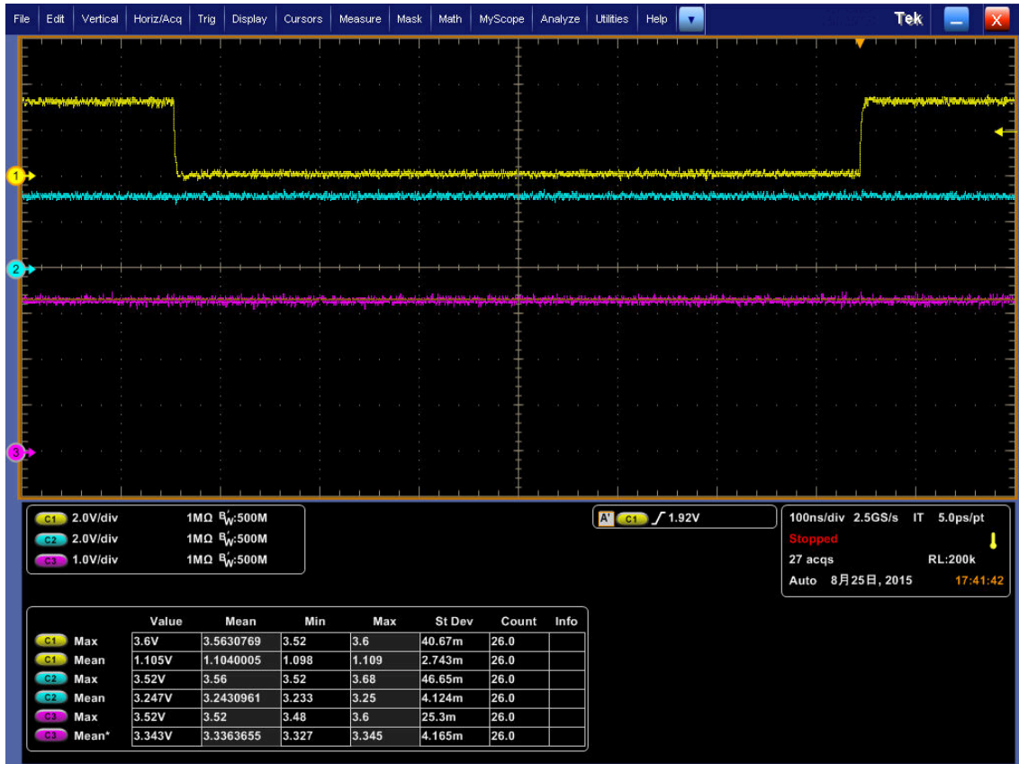
Fig. 6. OUT1 (CH1) , OUT2 (CH2) , REF 端子 (CH3) 電圧波形 (横軸 100nsec./div.)
