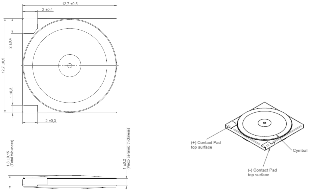
Fig. 1: Dimensional drawings
