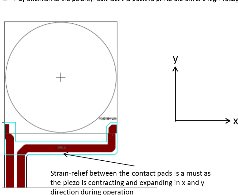
Fig. 12: Example of PowerHap with flexible PCB contact element.
