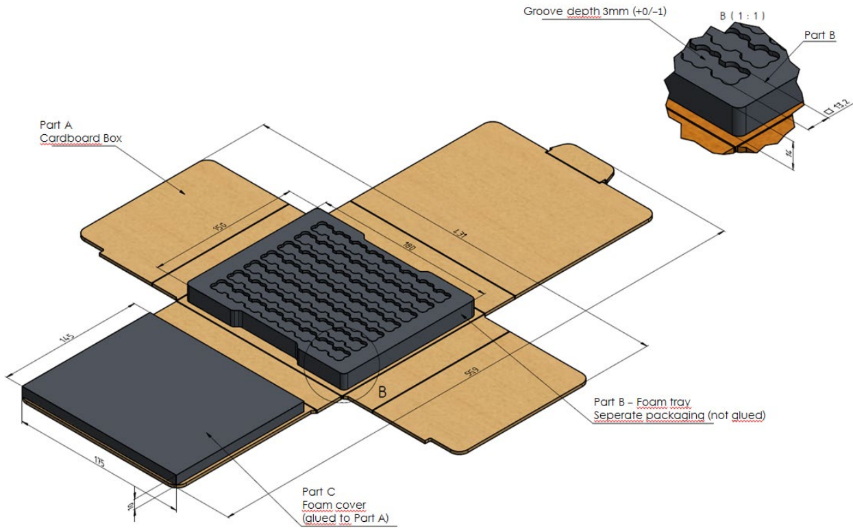
Fig. 18: Drawing of the packaging unit.
