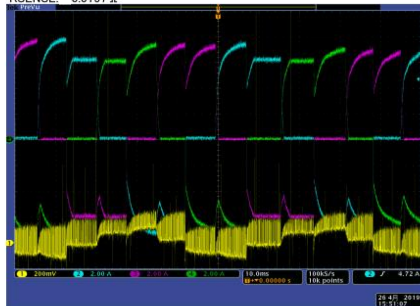
④ VDS 18k \Omega ( \pm 5\% ) to DVDD RSENSE: 0.0078 \Omega
