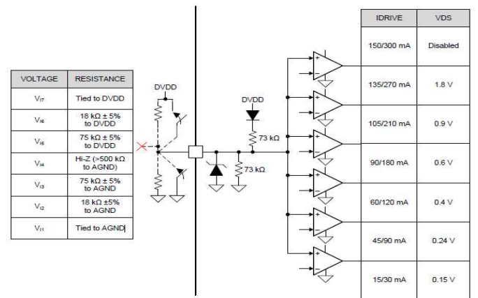
Figure 25. Seven Level Input Pin Structure
