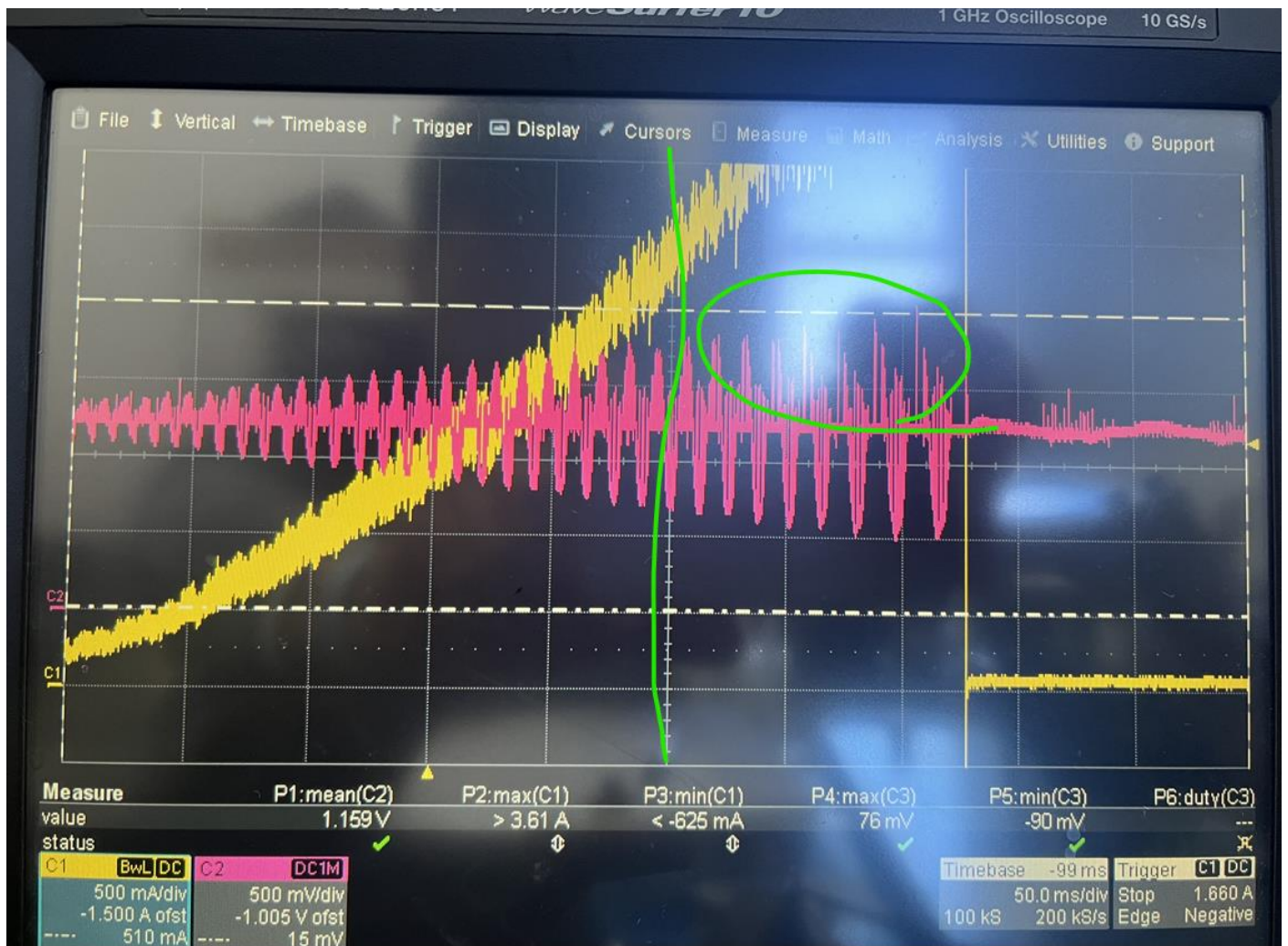
SOA/SOB/SOC output waveform
