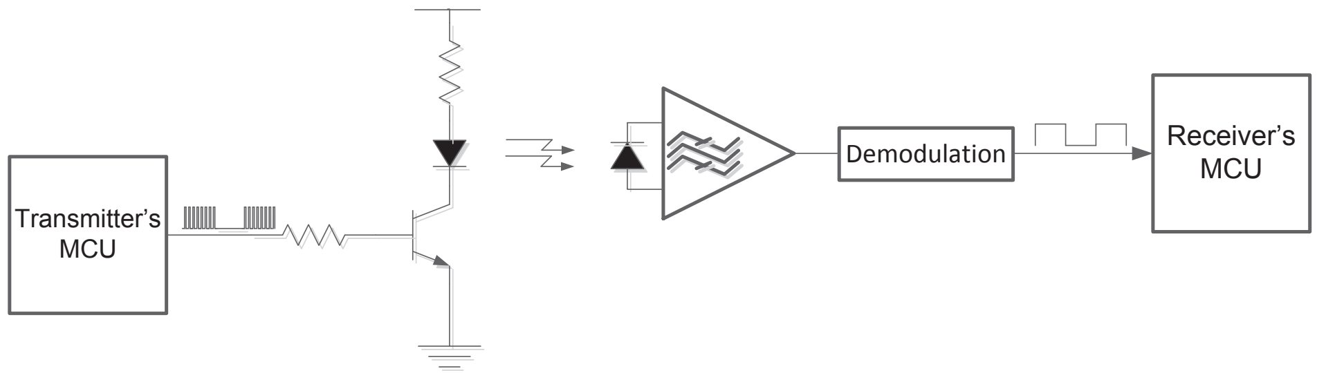
Figure 1. Infrared Modulation and Demodulation
