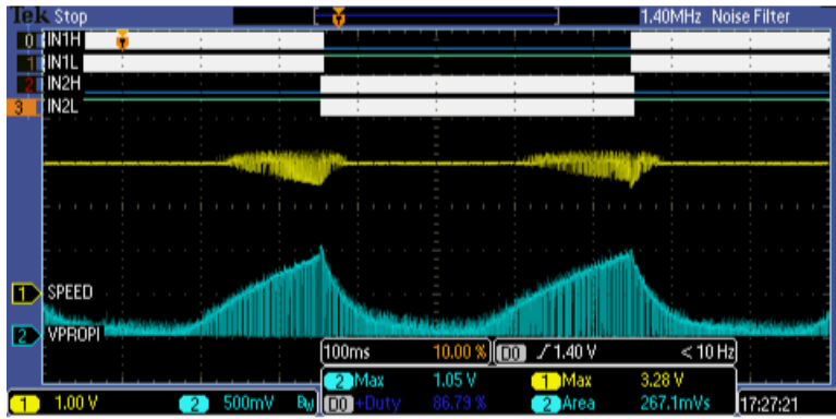
SFF-180SHV-2853_DRV8850_PWM-3
