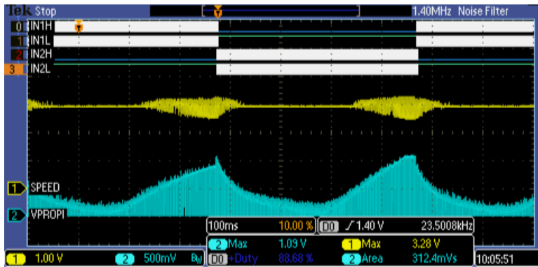
SFF-180SHV-3048_DRV8850_PWM
