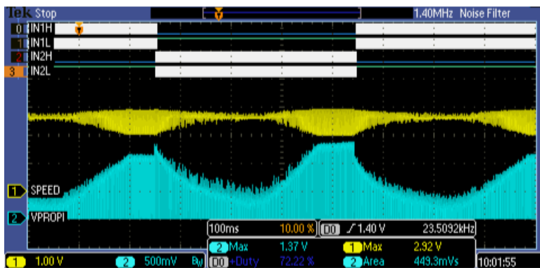
SFF-180SHV-3735_DRV8850_PWM
