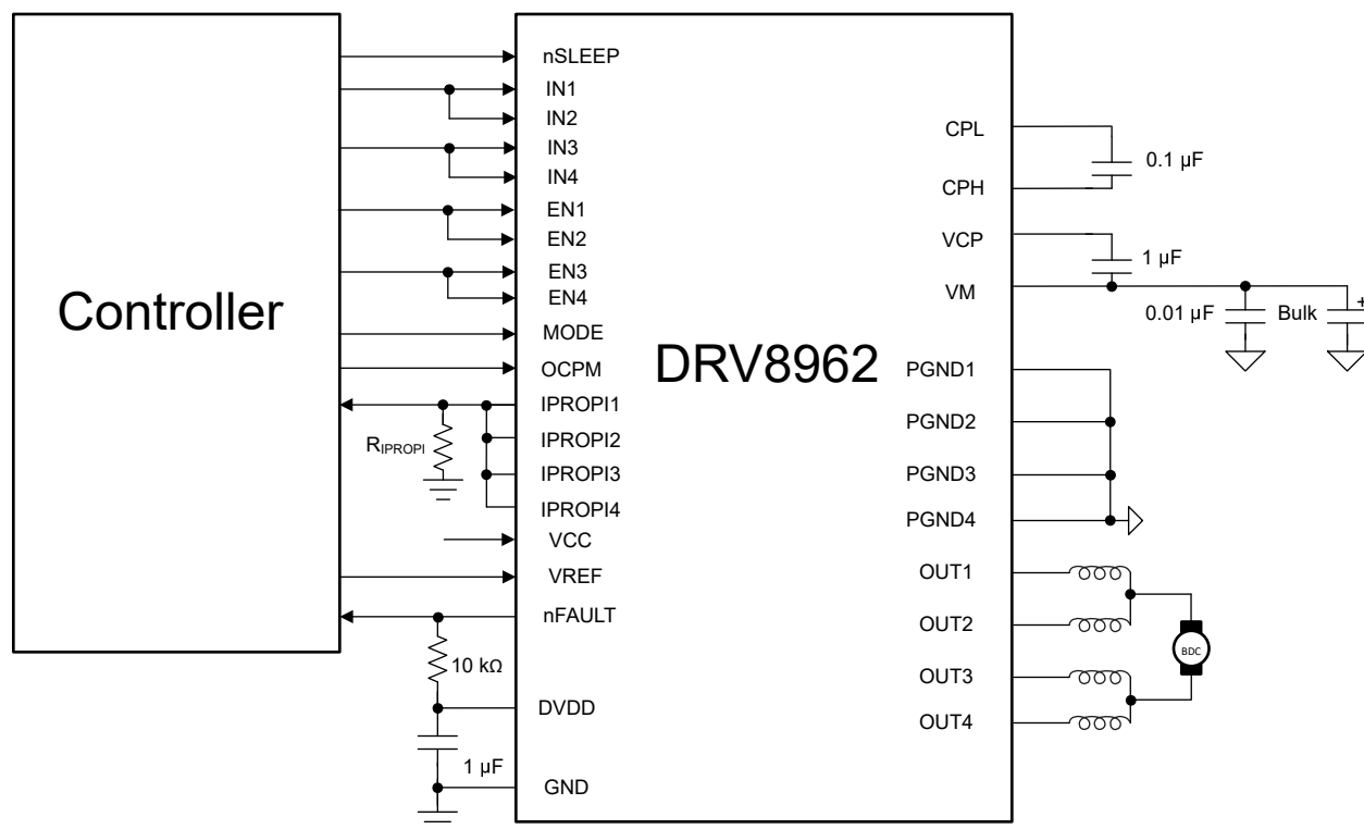
Figure 8-7. Driving Single Brushed-DC motor with DRV8962
