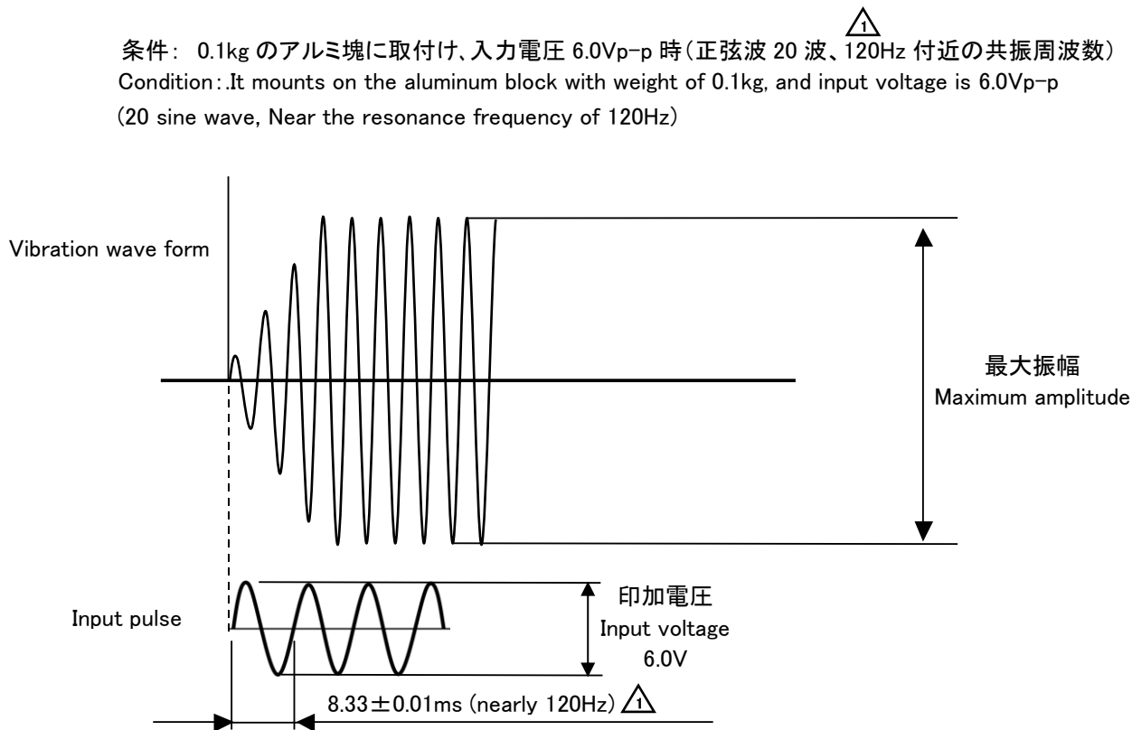
入力パルスと振動波形の関係 Relation between input pulse and vibration wave form
