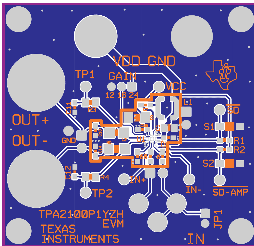
Figure 2. TPA2100P1 – YZH Package – Top Layer
