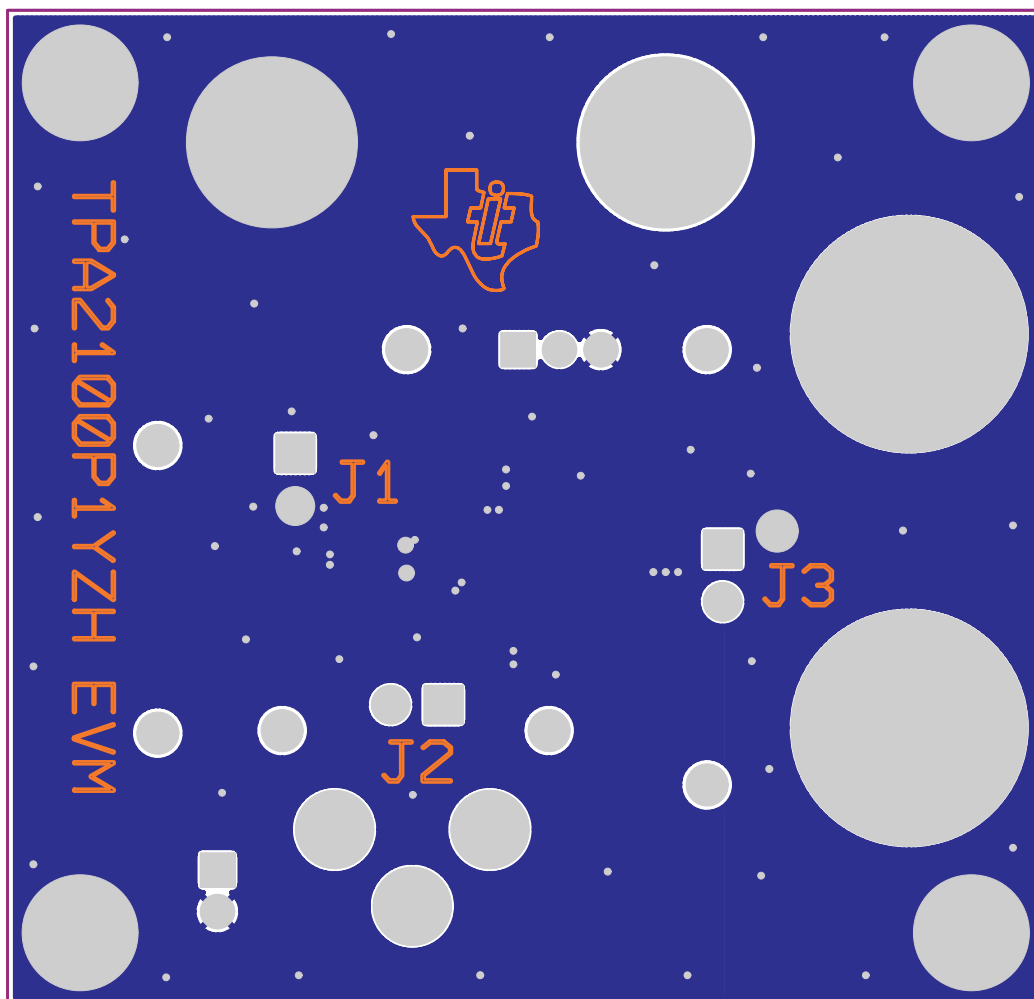
Figure 3. TPA2100P1 – YZH Package – Bottom Layer
