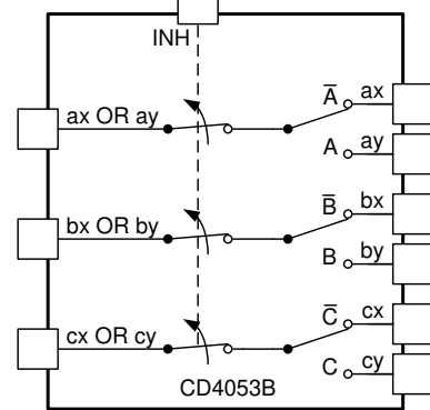
Functional Diagrams of CD405xB
