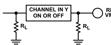
Figure 7-15. Crosstalk Between Duals or Triplets (CD4052B, CD4053B)
