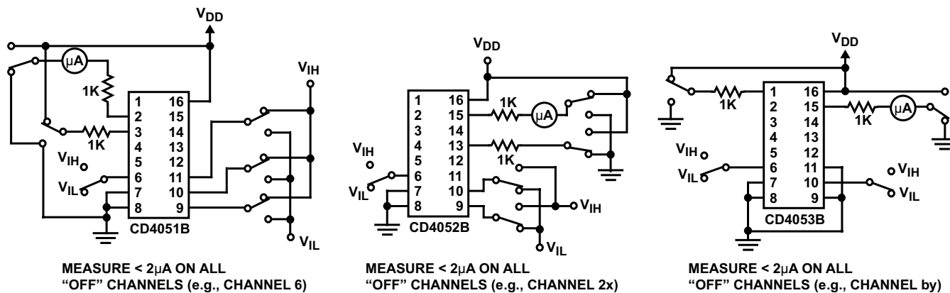
Figure 16. Input Voltage Test Circuits (Noise Immunity)
