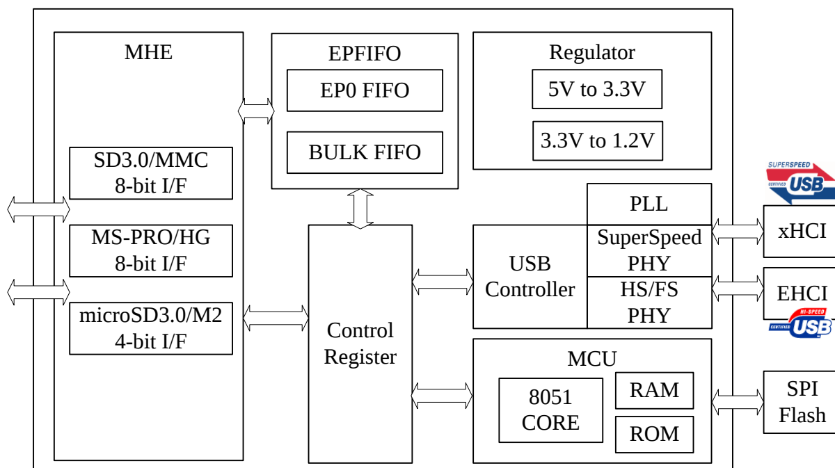
Figure 4.1 – QFN48 Functional Block Diagram
