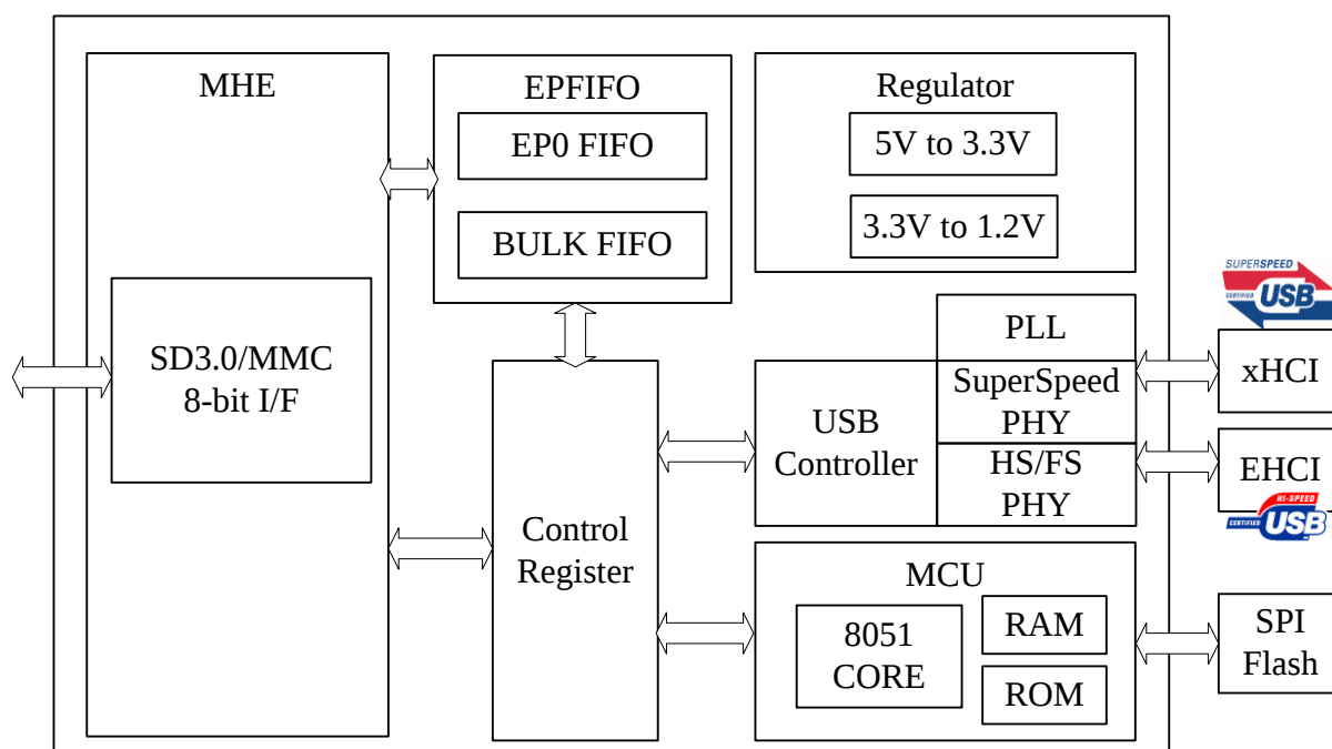
Figure 4.2 – QFN32 Functional Block Diagram
