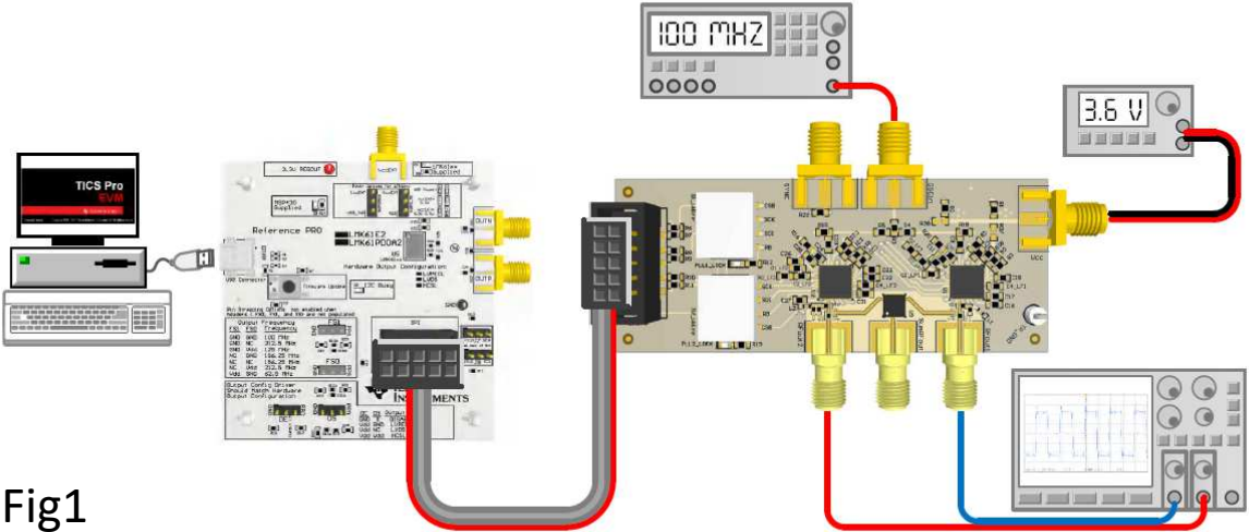
Figure 2-1. Connection Diagram
