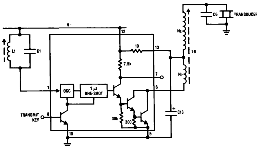
FIGURE 5. Transmitter
