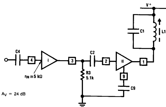
FIGURE 9. Receiver Section
