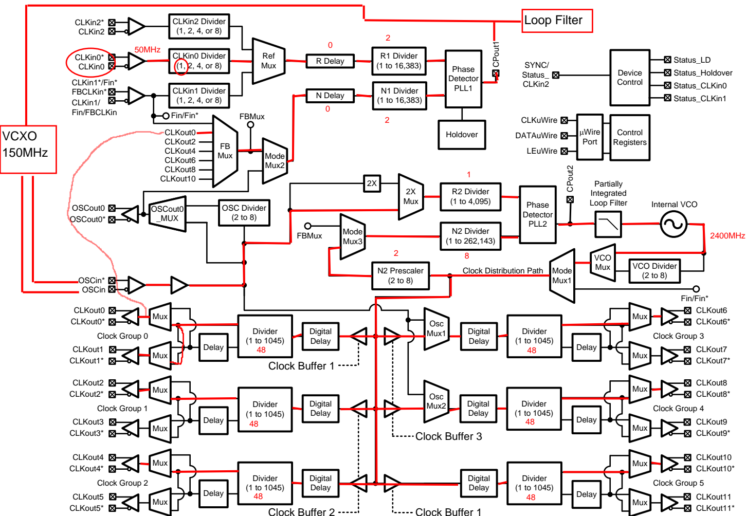
Figure 2-6. Detailed LMK04816 Block Diagram
