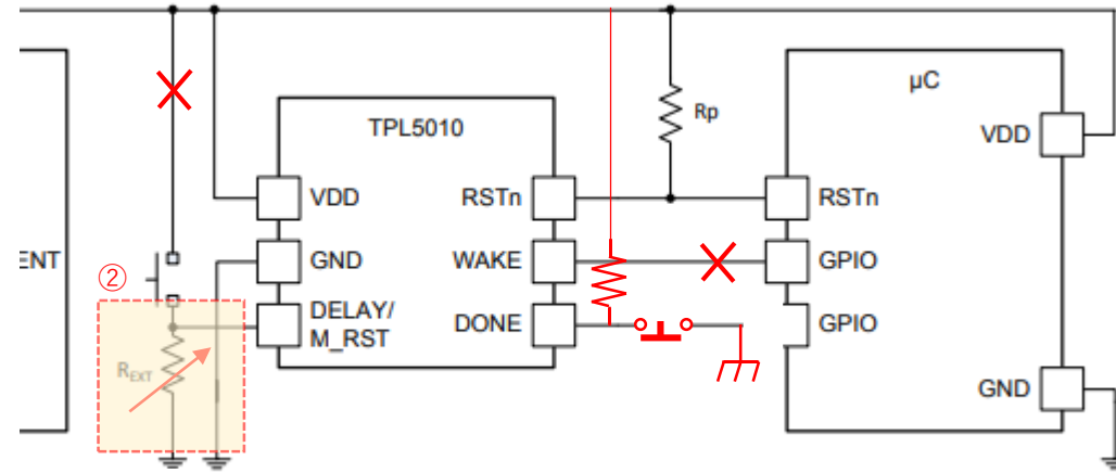
TPL0401 1. Manual Reset with SPST Switch
