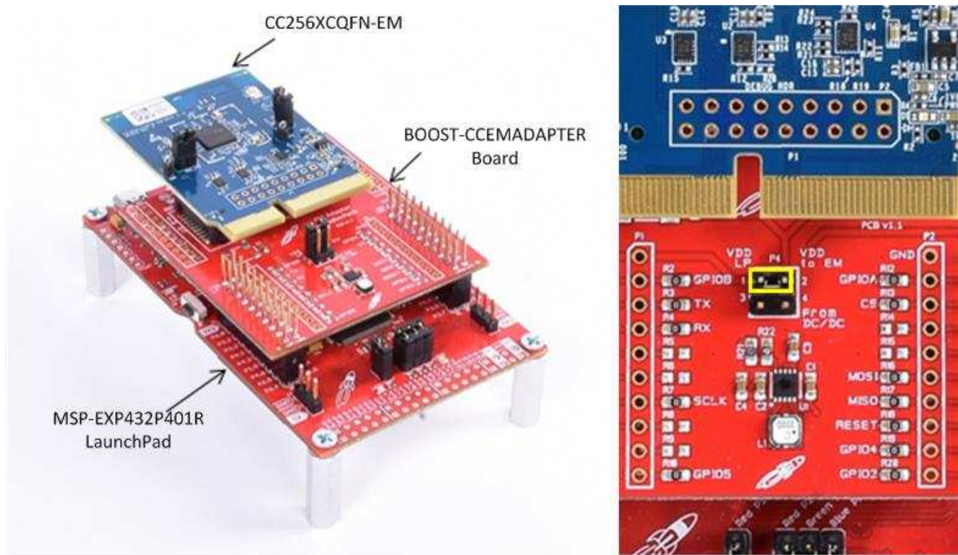
Figure 2. Hardware Requirement Combinations
