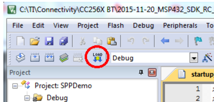
Figure 16. LOAD Button
