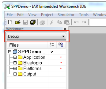
Figure 9. Debug Workspace
