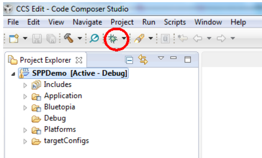
Figure 7. Debug Icon
