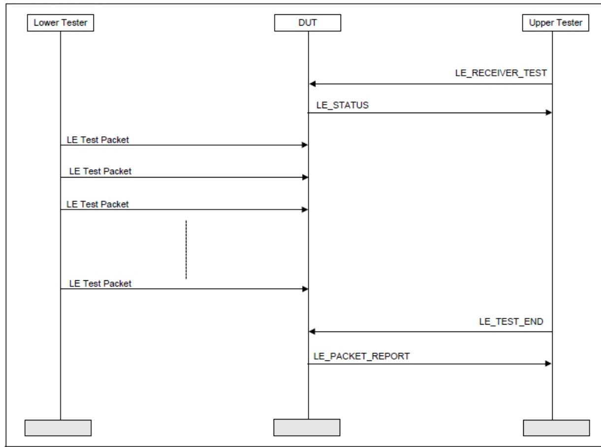
Figure 2.2: Receiver Test MSC
