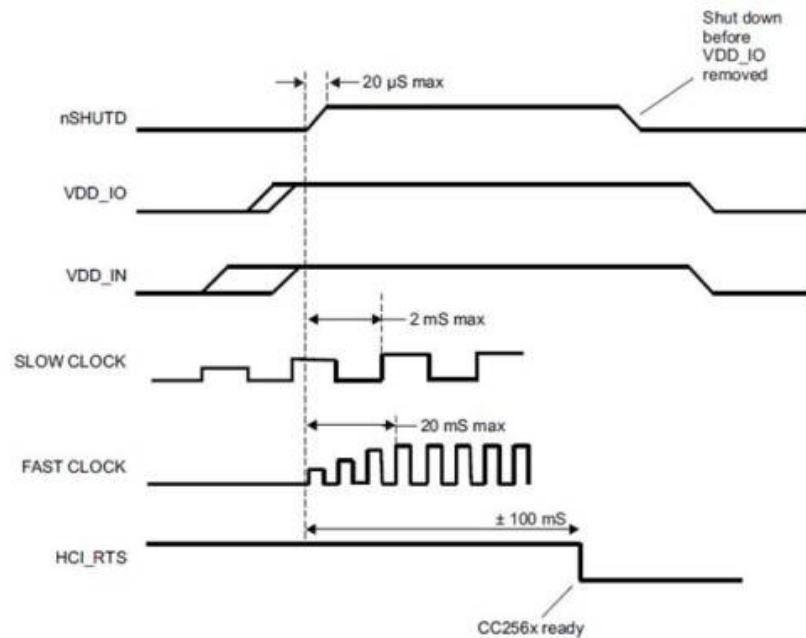
Figure: Proper Power Up Sequence
