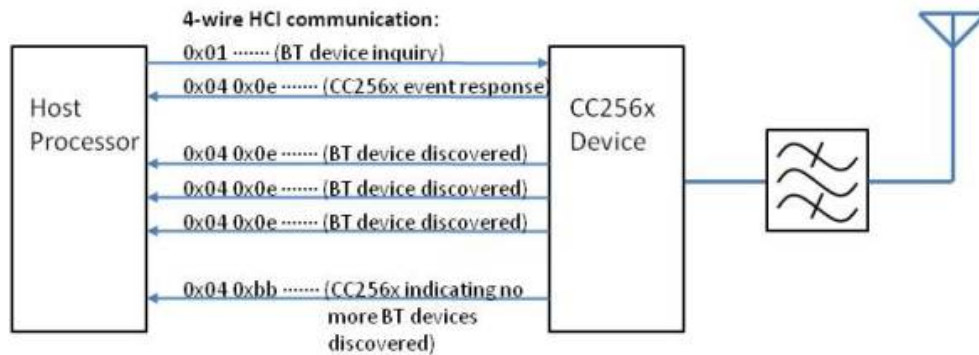
Figure: Example of Bluetooth Inquiry Operation
