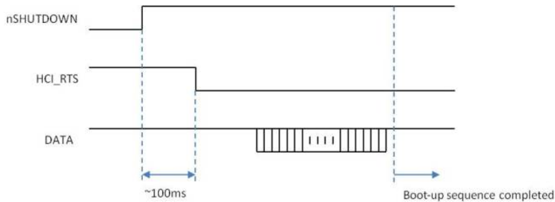
Figure: Device Initialization Sequence
