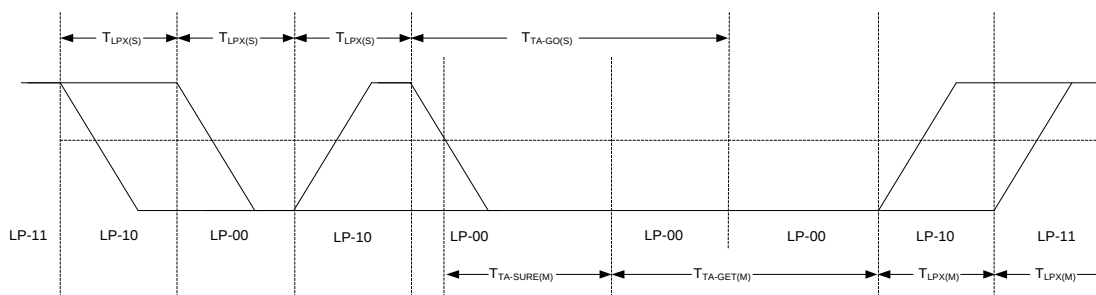
Figure 9.7-4. Turnaround procedure from display module to MCU
