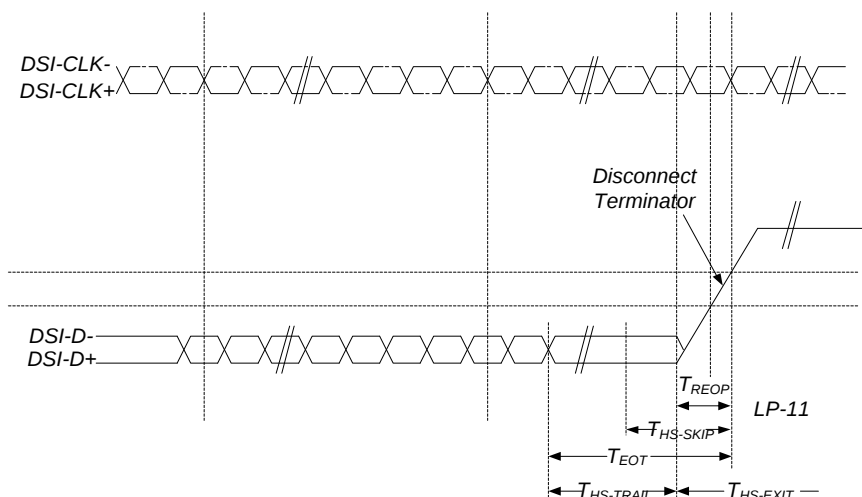
Figure 9.7-2. HS data transmission in bursts
