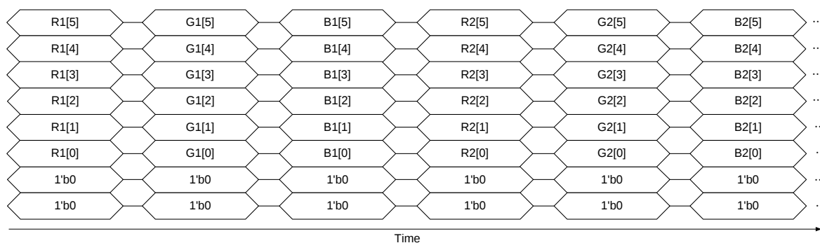
Figure 9.8-2. Pixel format of loose RGB666
