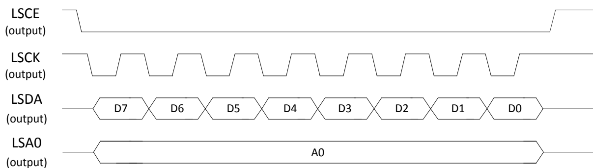
Figure 9.6-3. 4-wire serial interface write (8-bit)
