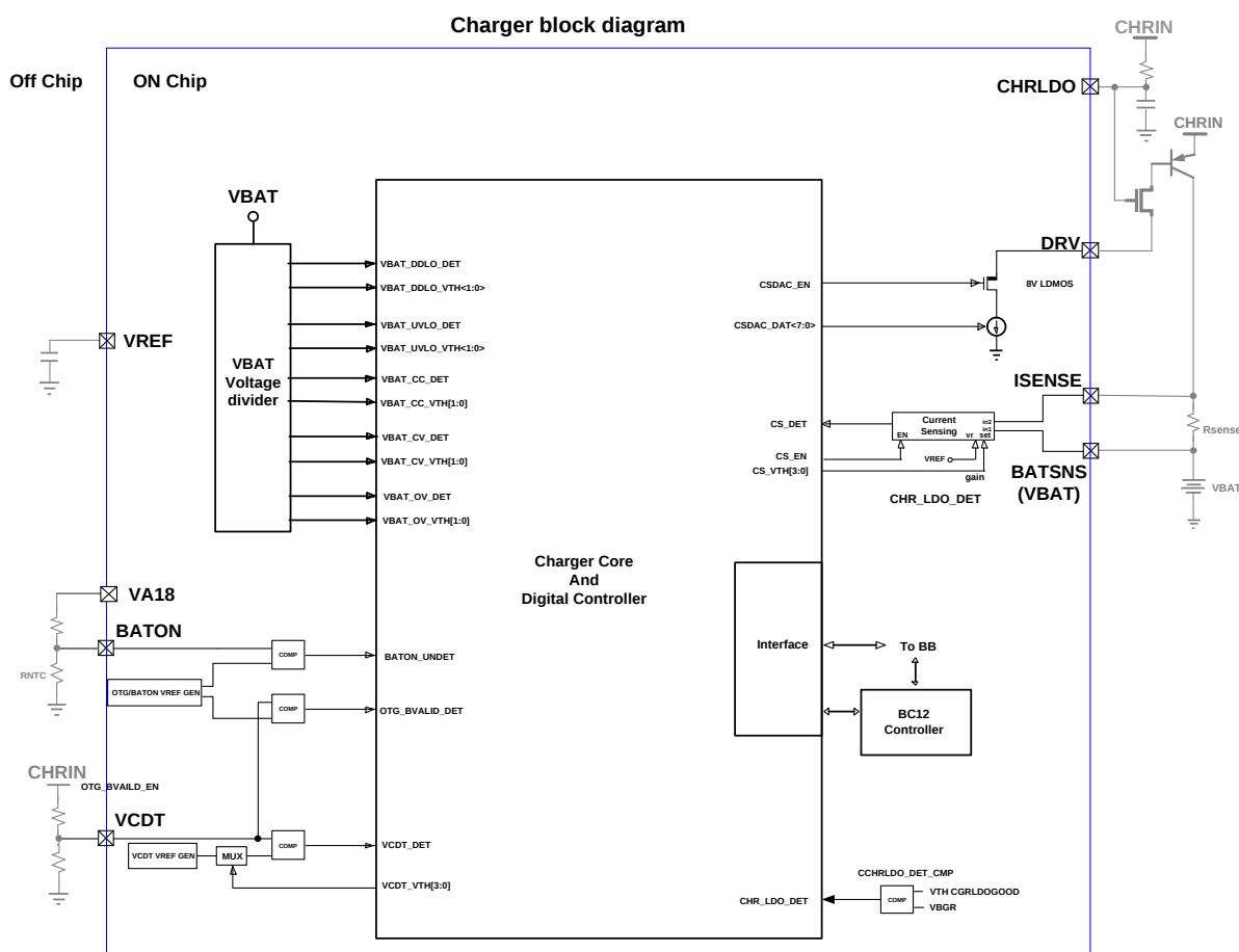
Figure 5.4-1. PCHR schematics
