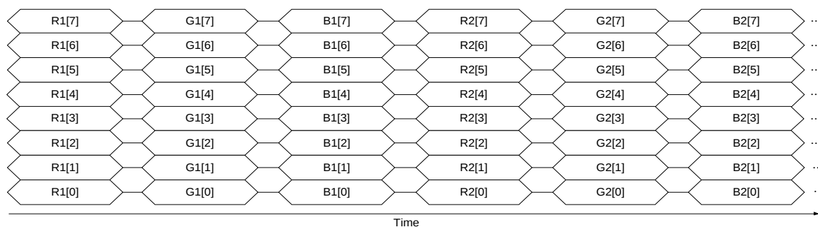
Figure 9.8-1. Pixel format of RGB565
