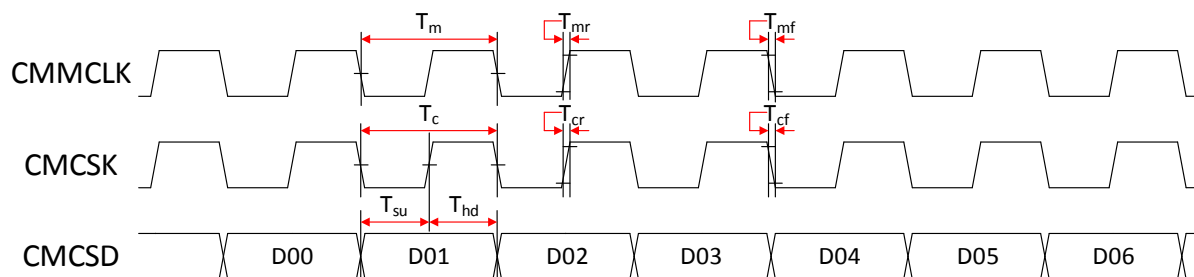
Figure 9.9-2. I/O port timing of SDR mode
