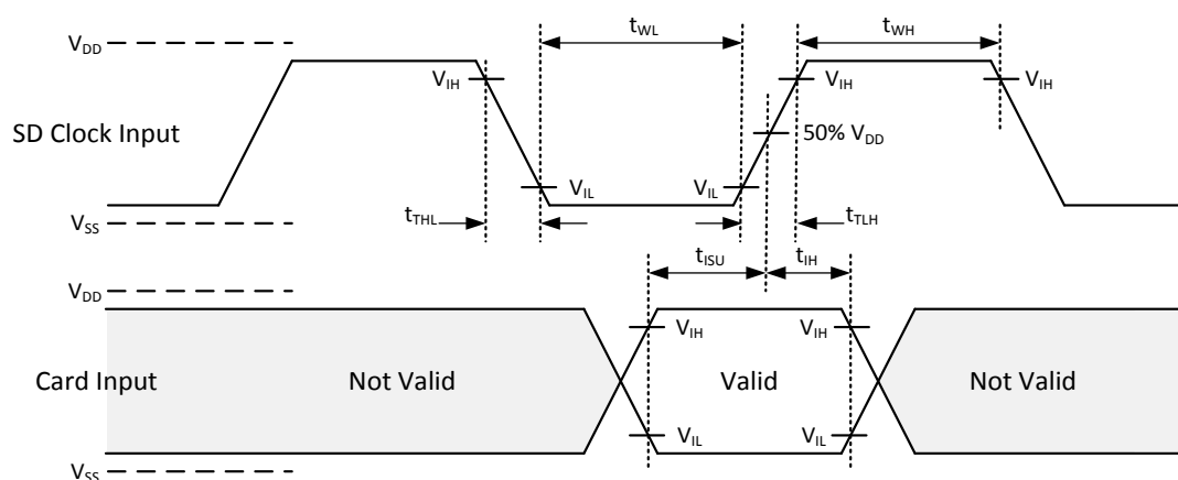
Figure 9.3-9. SD controller input timing (high-speed mode)
