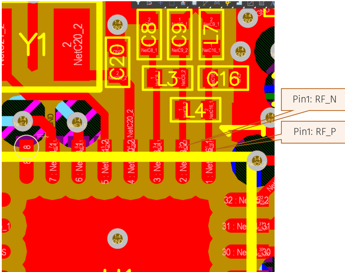
Top layer showing RF_P and RF_N pins
