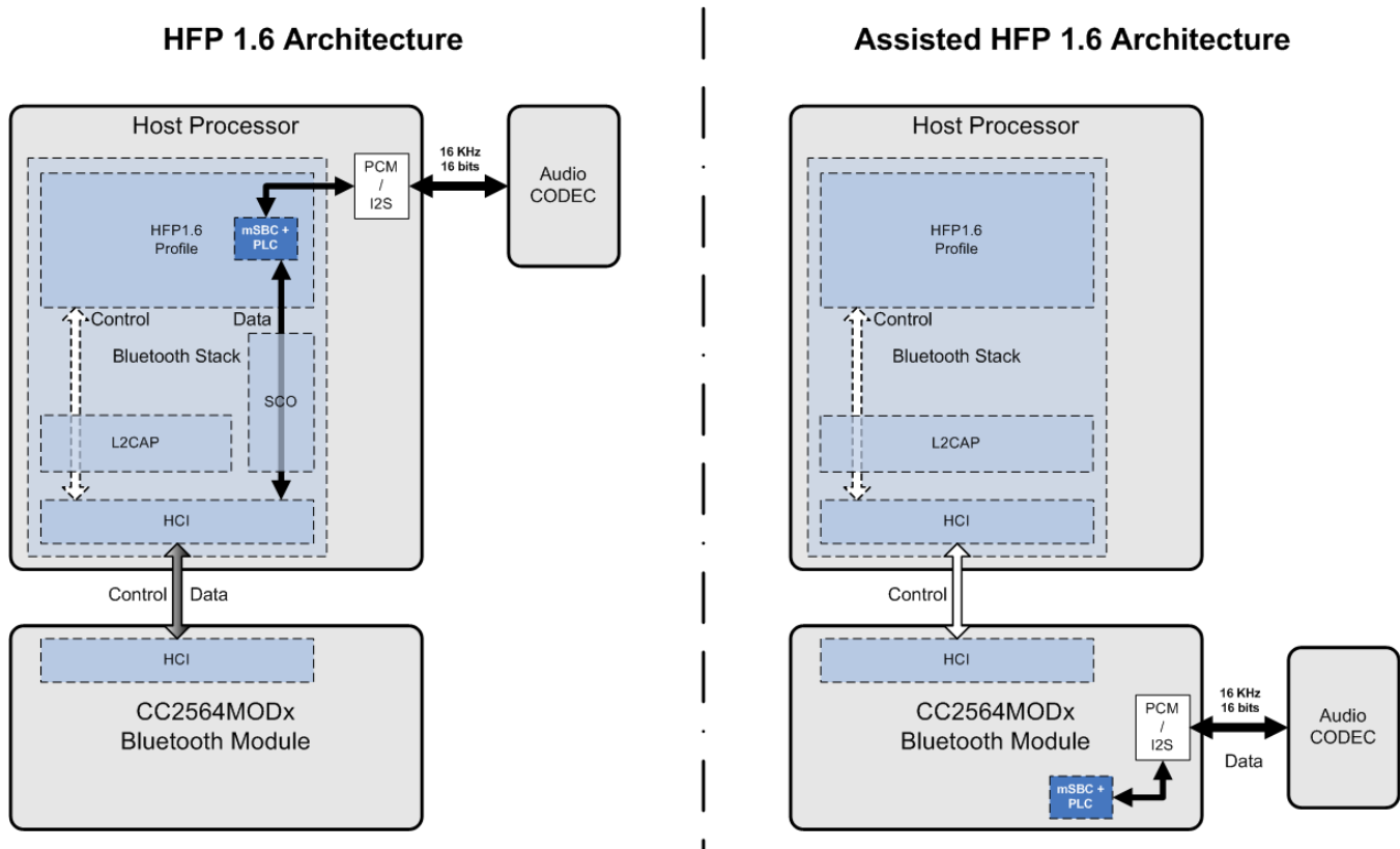
Figure 5-9. HFP 1.6 Architecture Versus Assisted HFP 1.6 Architecture
