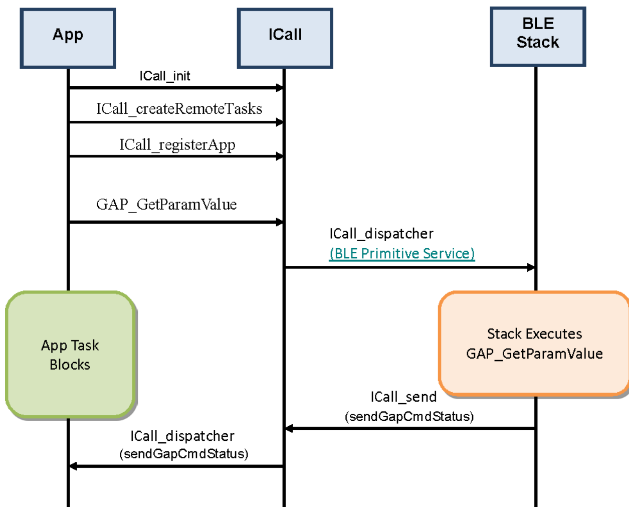
Figure 4-2. ICall Messaging Example
