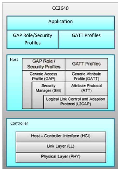
Figure 2-2. Single-Device Processor Configuration
