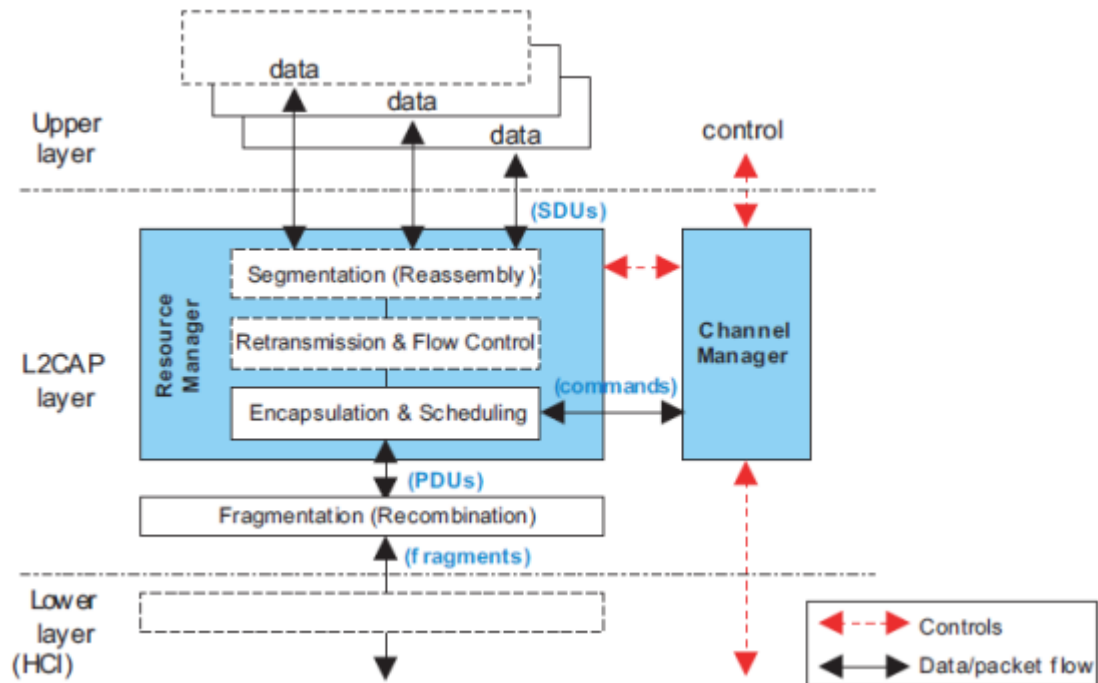
Figure 5-25. L2CAP Architectural Blocks
