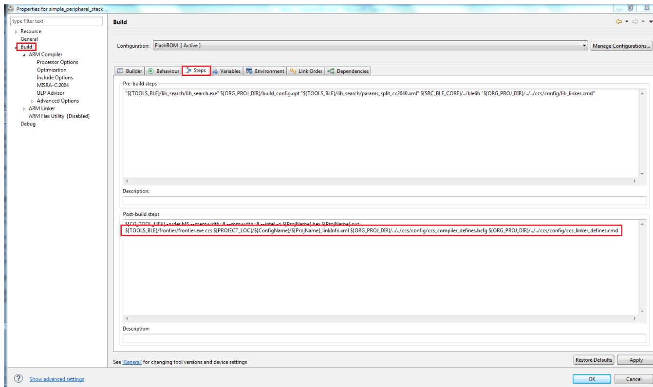
Figure 3-9. Disabling Frontier Tool from Stack Project in CCS
