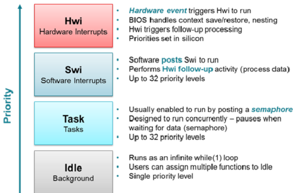
Figure 3-1. RTOS Execution Threads
