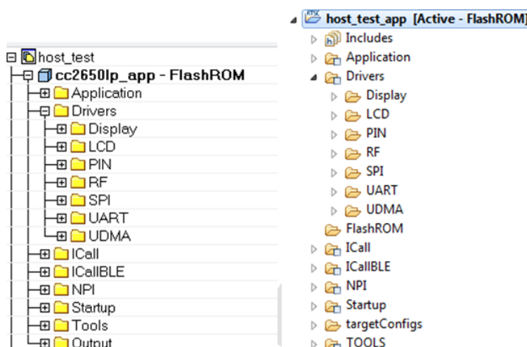
Figure 6-1. Drivers Folder
