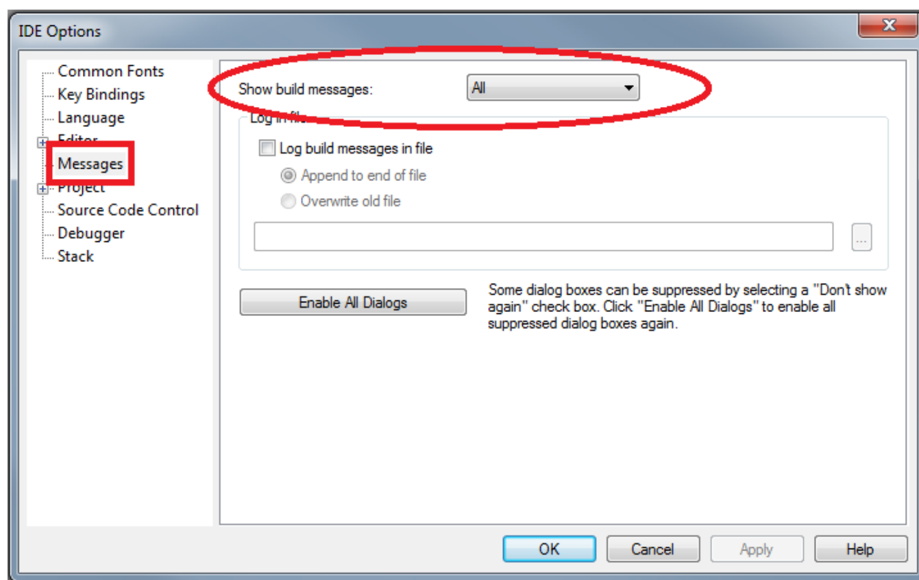
Figure 2-5. Full Verbosity
