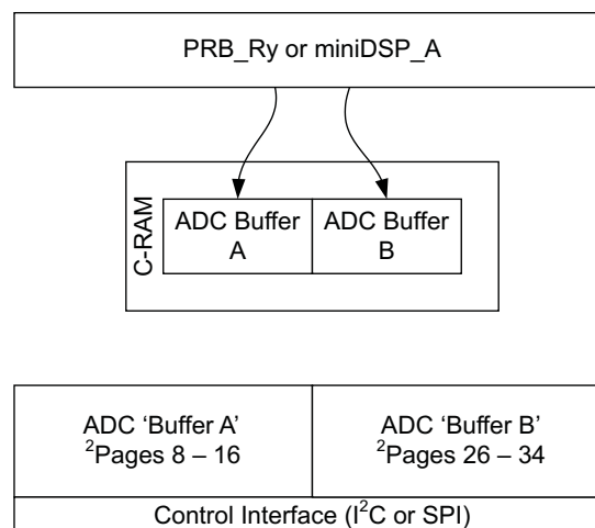
Figure 8. ADC C-RAM Access at Power-Down and Power-Up Modes – Nonadaptive
