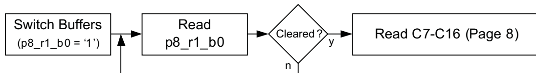
Figure 12. Reading ADC C-RAM Coefficients in Adaptive Mode Example – AIC32x4
