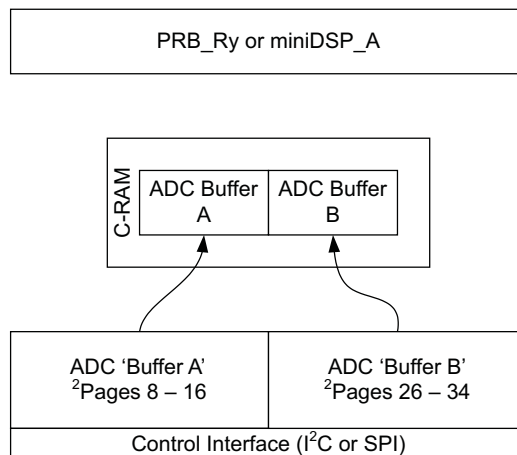
Figure 9. ADC C-RAM Access at Power-Down Mode – Adaptive
