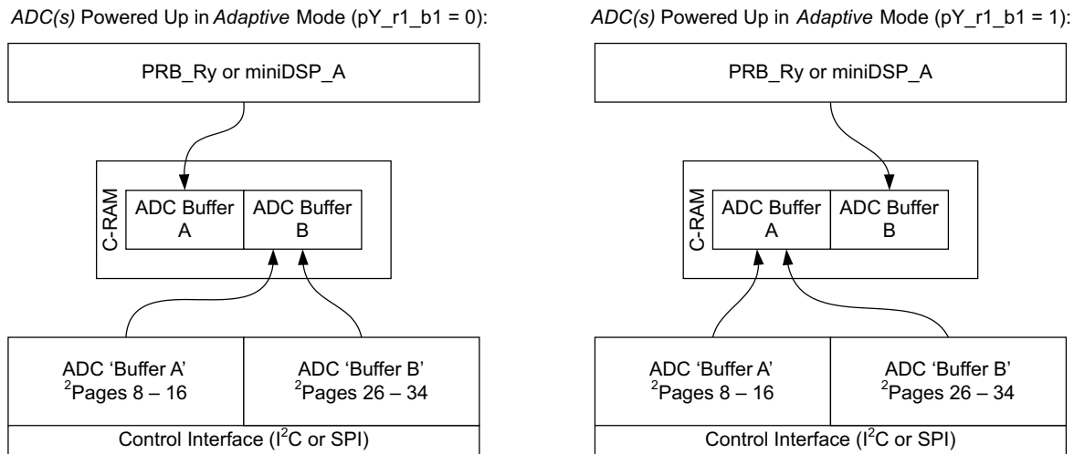
Figure 10. ADC C-RAM Access at Power-Up Mode – Adaptive
