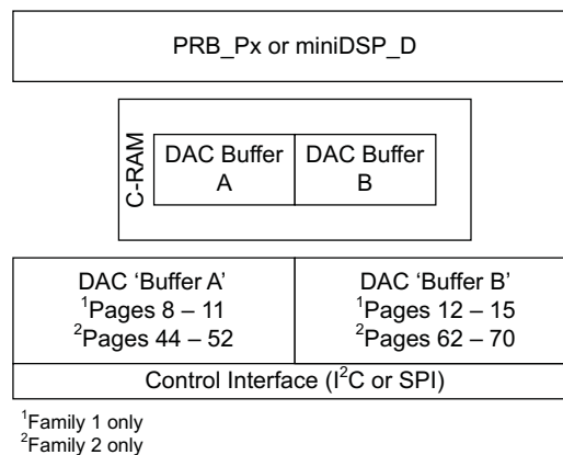
Figure 1. Components Related to DAC C-RAM Access
