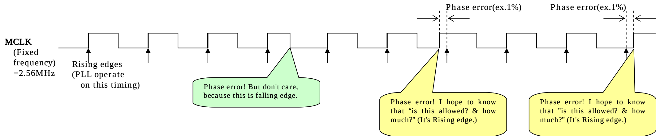
Fig.1 MCLKs (fixed frequency but includes phase error)
