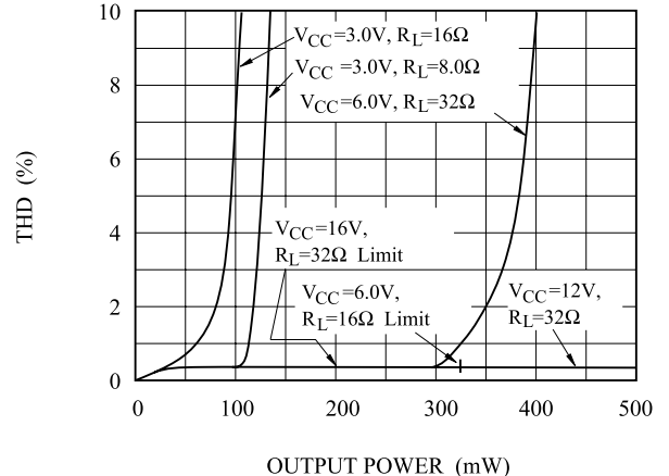
FIGURE13-DISTORTION versus POWER f=1,3.0kHz,AVD=12dB
