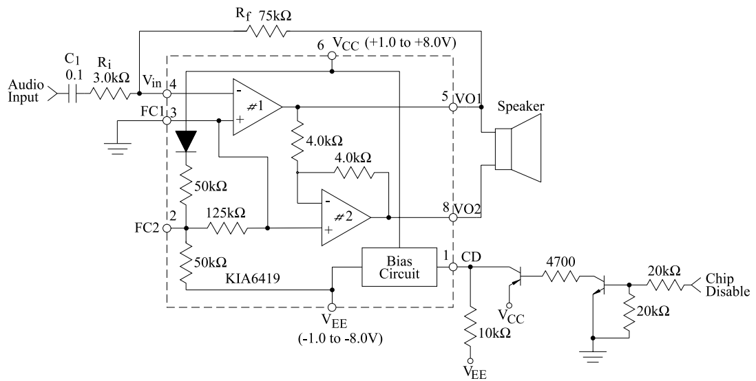
FIGURE26-SPLIT SUPPLY OPERATION
