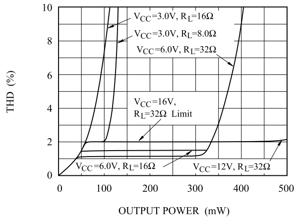
FIGURE12-DISTORTION versus POWER f=3.0kHz,AVD=34dB
