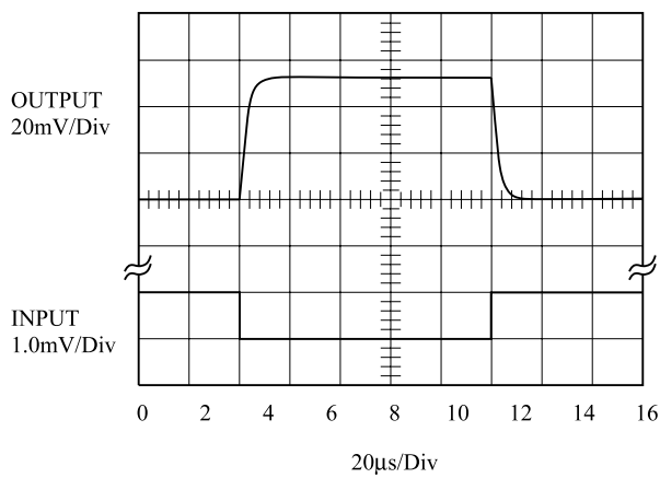
FIGURE16-SMALL SIGNAL RESPONSE
