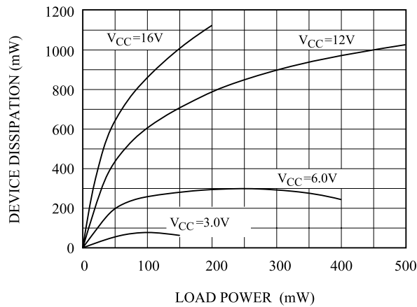
FIGURE10-DEVICE DISSIPATION 32Ω LOAD
