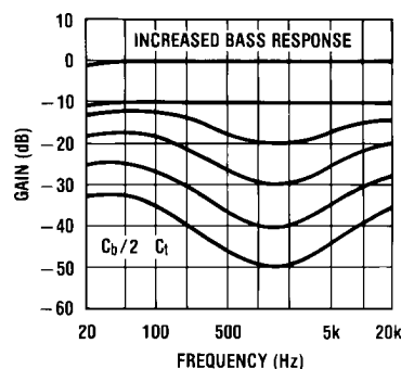
FIGURE 8. Loudness Compensated Volume Characteristic
