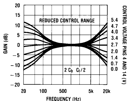
FIGURE 4. Tone Characteristic (Gain vs Frequency)
