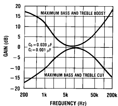
FIGURE 15. Tone Characteristic (Gain vs Frequency)
