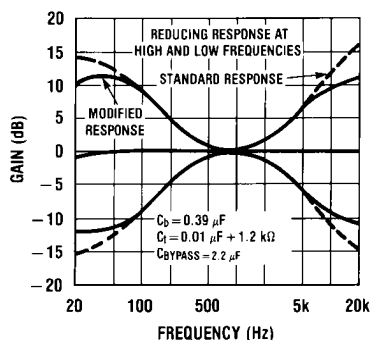
FIGURE 6. Tone Characteristic (Gain vs Frequency)
