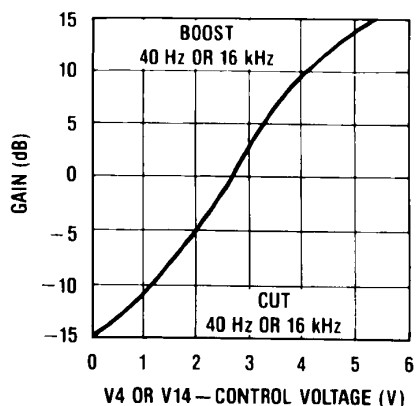
Tone Control Characteristic
