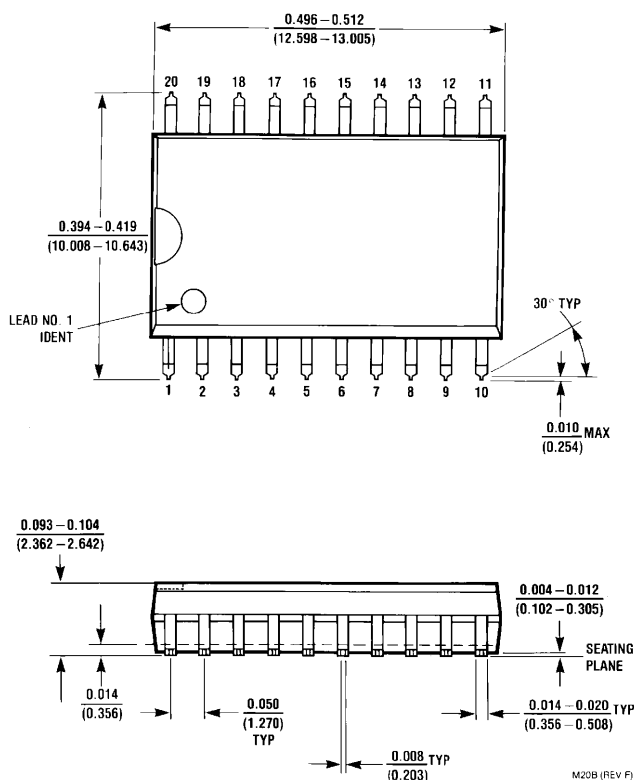
Small Outline (SO) Package Order Number LM1036M or LM1036MX NS Package Number M20B
