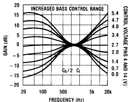
FIGURE 5. Tone Characteristic (Gain vs Frequency)
