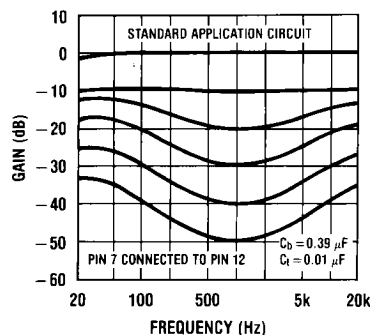
FIGURE 7. Loudness Compensated Volume Characteristic
