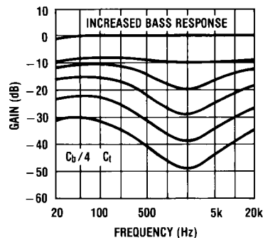
FIGURE 9. Loudness Compensated Volume Characteristic
