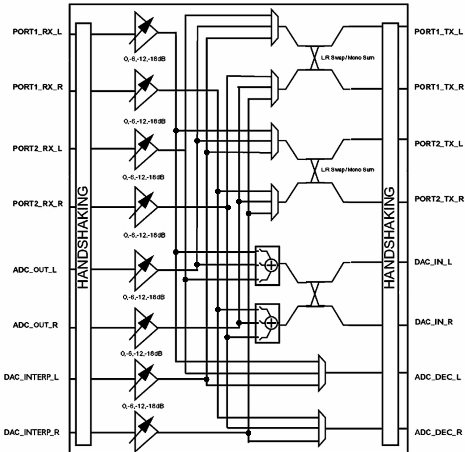
Figure 61. Digital Mixer
