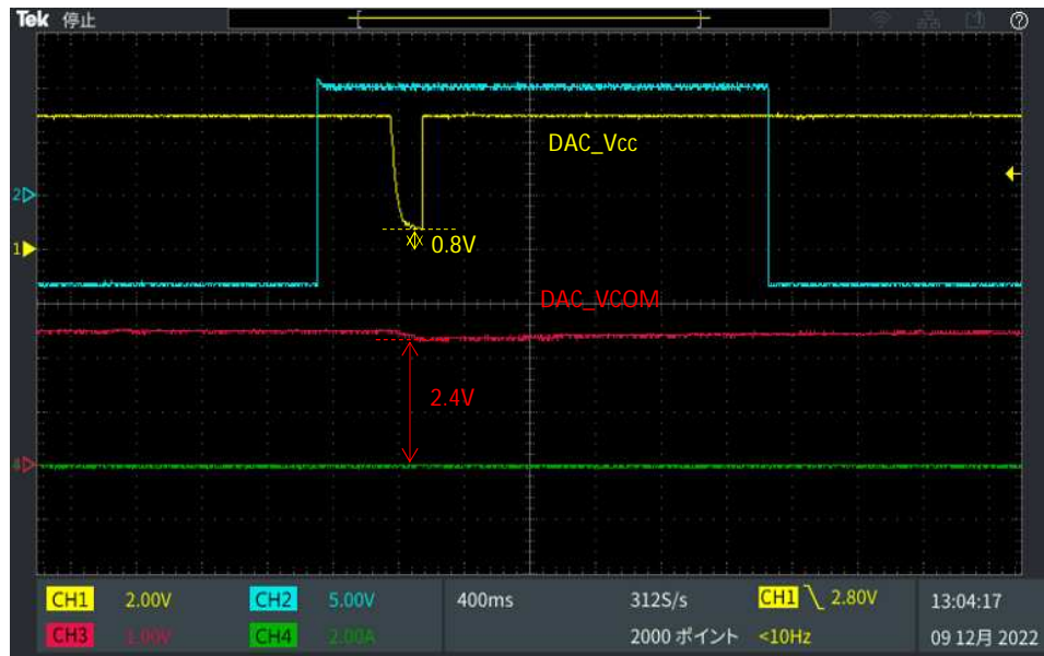
VCOM = 100uF Unstable SNR
