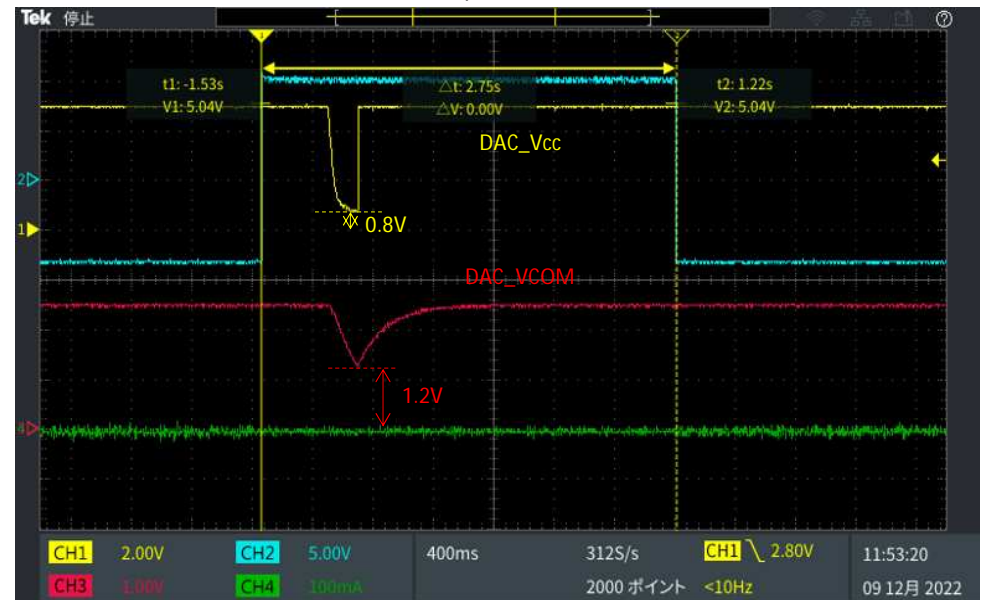
VCOM = 10uF Stable SNR performance
