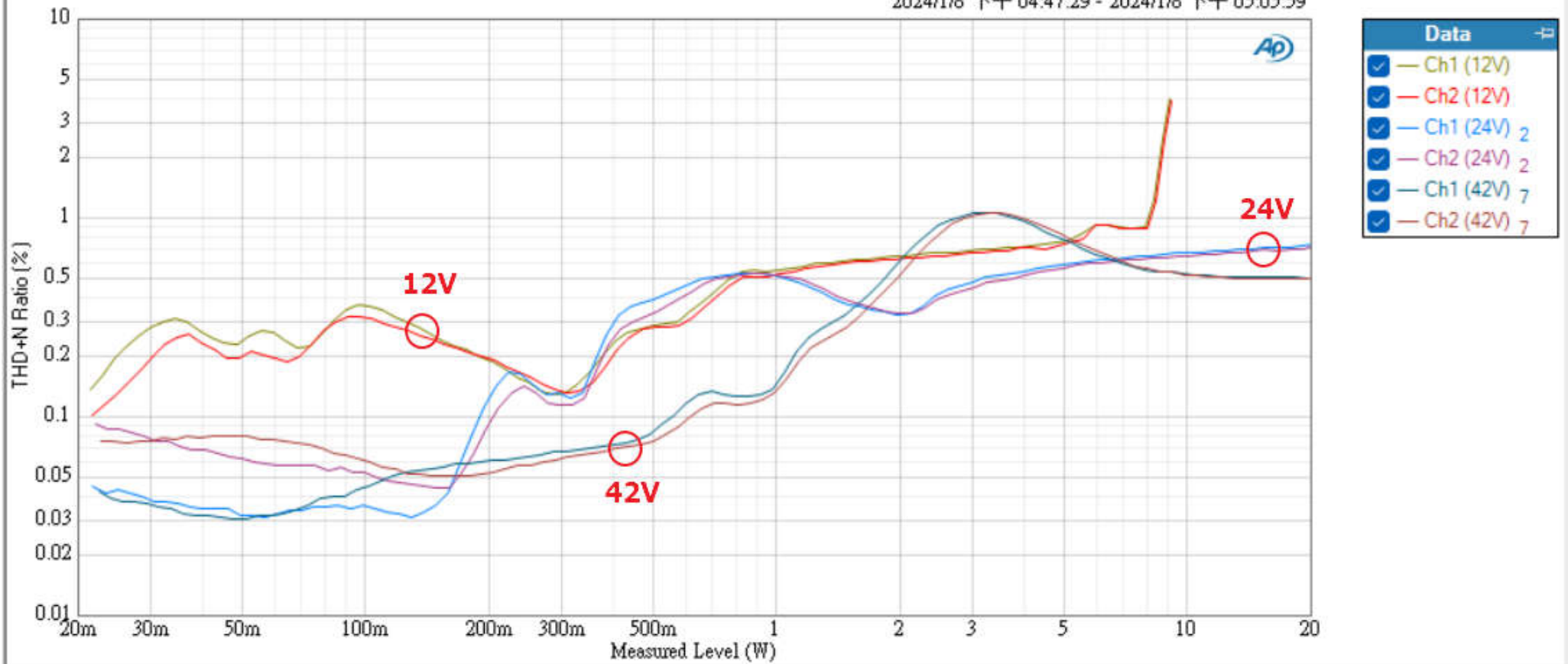
THD+N Ratio vs Measured Level
