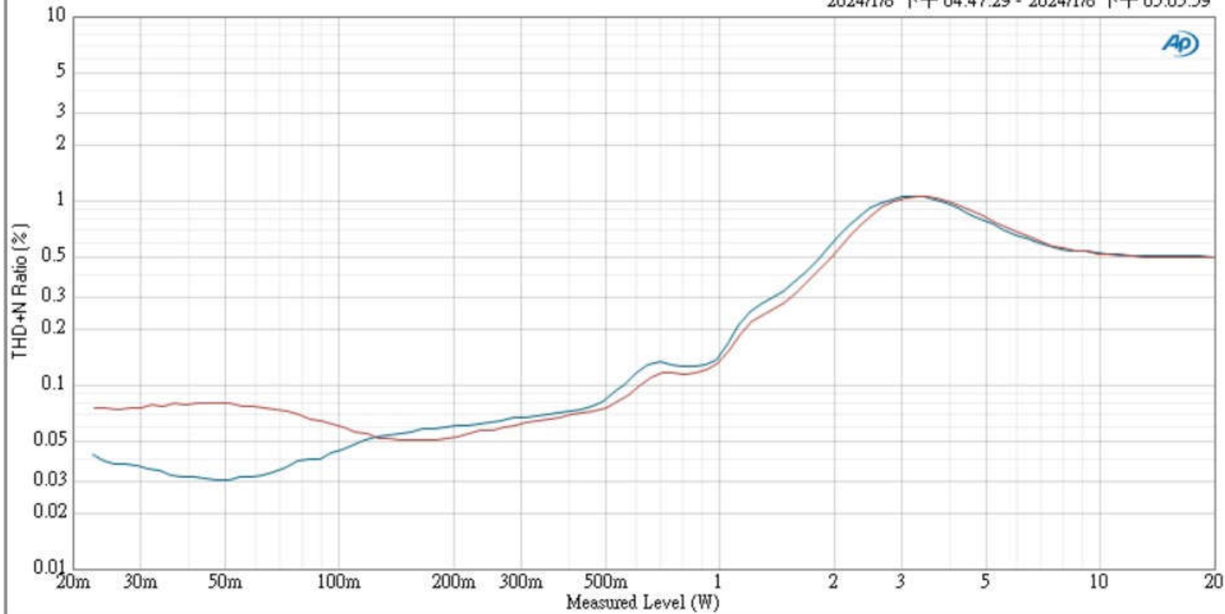
THD+N Ratio vs Measured Level
