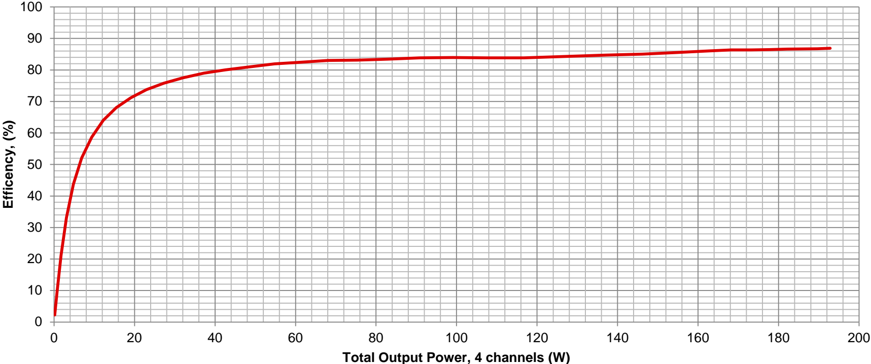
Efficiency vs Power, TAS5414C-Q1, 2 ohms
