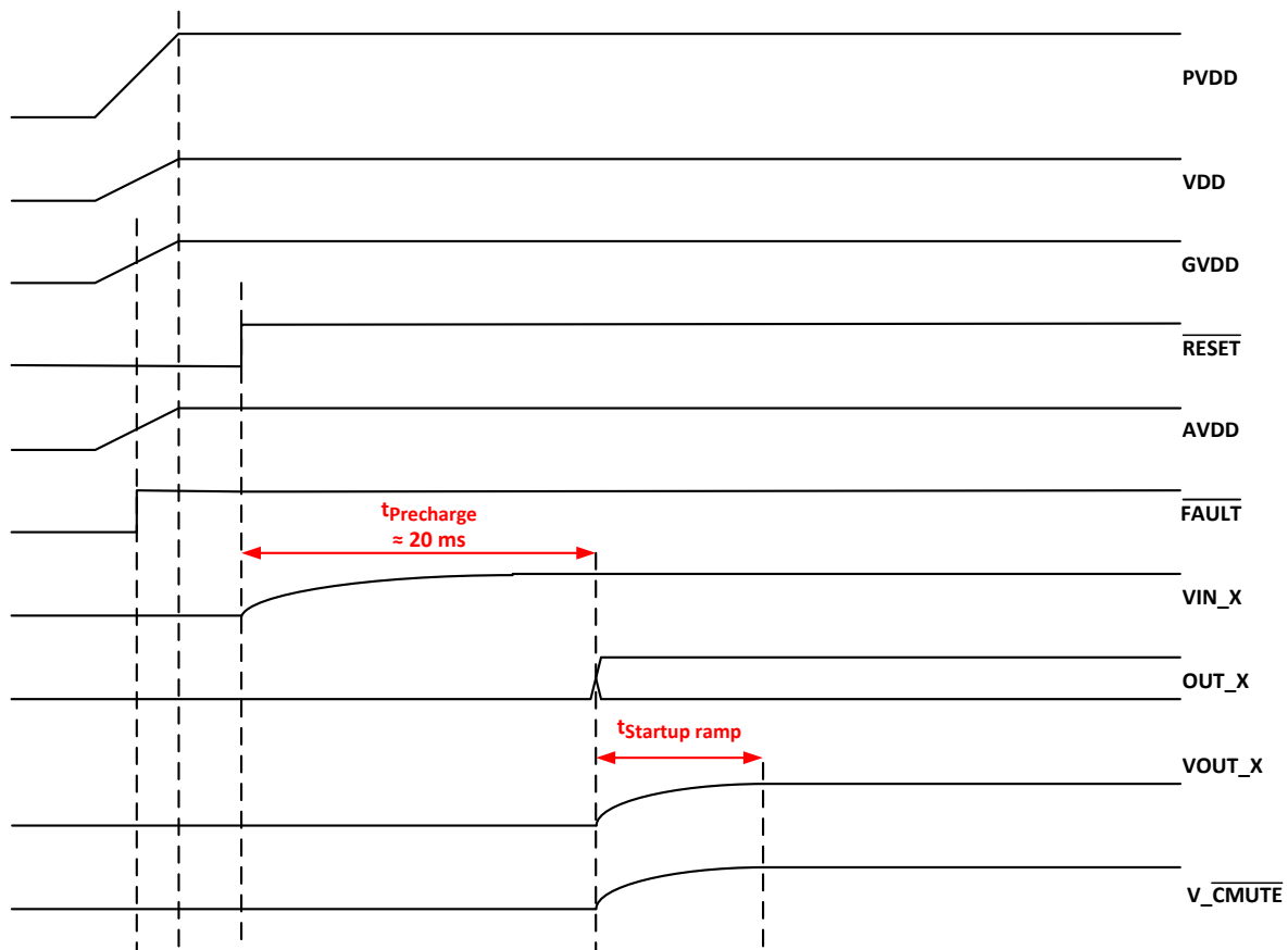
Figure 8-21. Startup Timing
