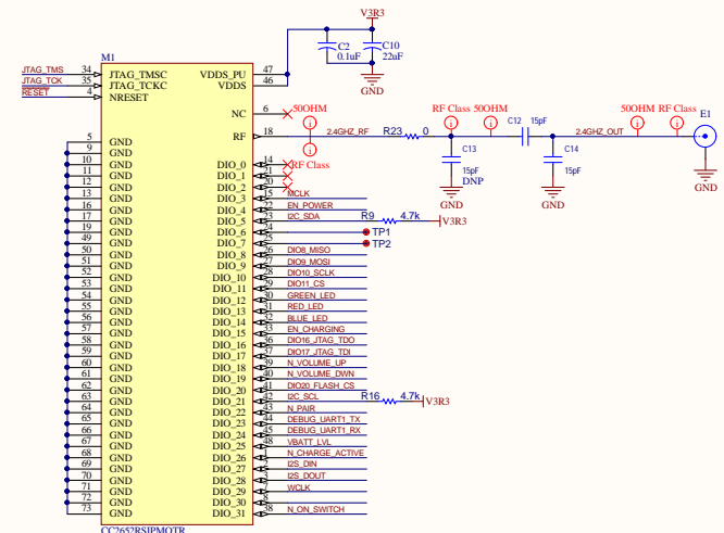
CC2652R5P4MOTR
