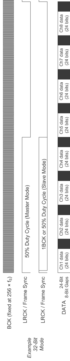
Figure 46. Audio Format for TDM
