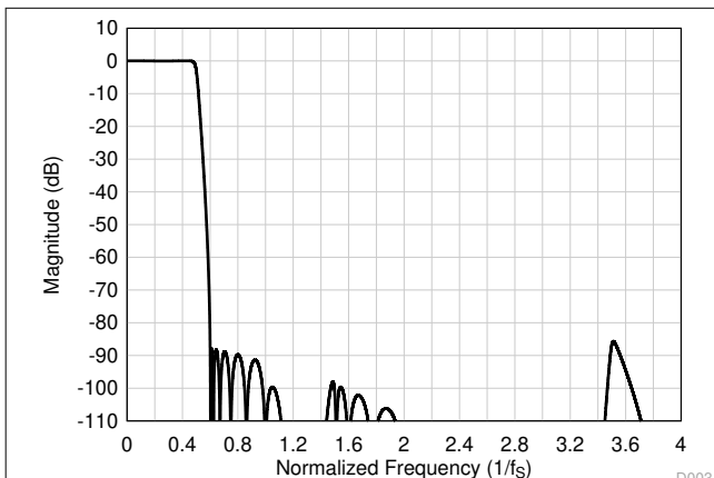
Figure 8-61. Ultra-Low-Latency Decimation Filter Magnitude Response
