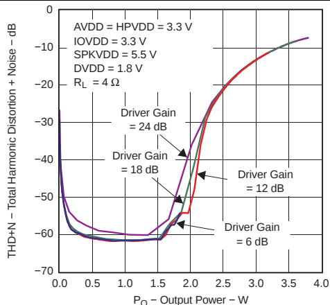
Figure 5-15. Total Harmonic Distortion + Noise vs Output Power Max Class-D Speaker-Driver Output Power ( R_L = 4 \Omega )
