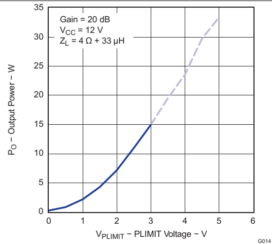
Figure 14. Output Power vs PLIMIT Voltage (BTL)
