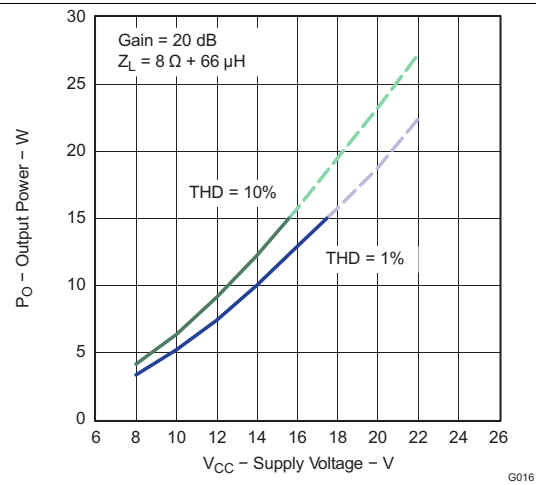
Figure 16. Output Power vs Supply Voltage (BTL)
