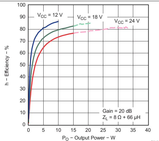
Figure 18. Efficiency vs Output Power (BTL)
