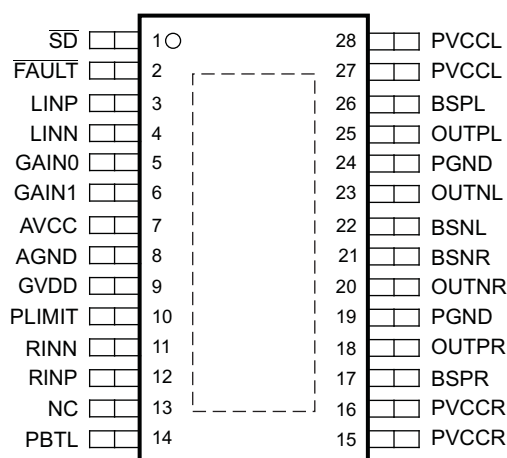
Pin Functions
