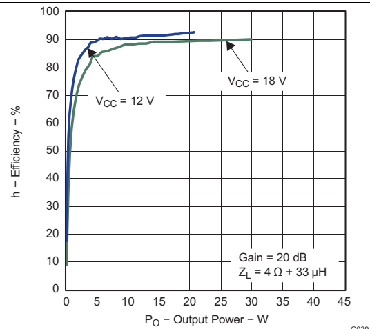
Figure 32. Efficiency vs Output Power (PBTL)
