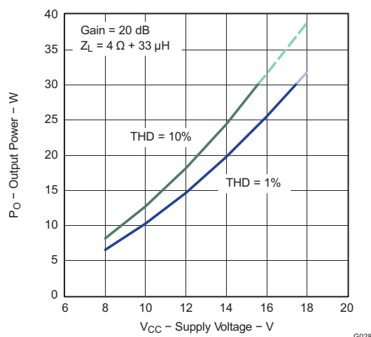
Figure 46. Output Power vs Supply Voltage (PBTl)
