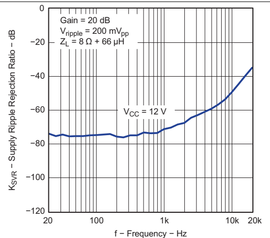
Figure 34. Supply Ripple Rejection Ratio vs Frequency (PBTL)
