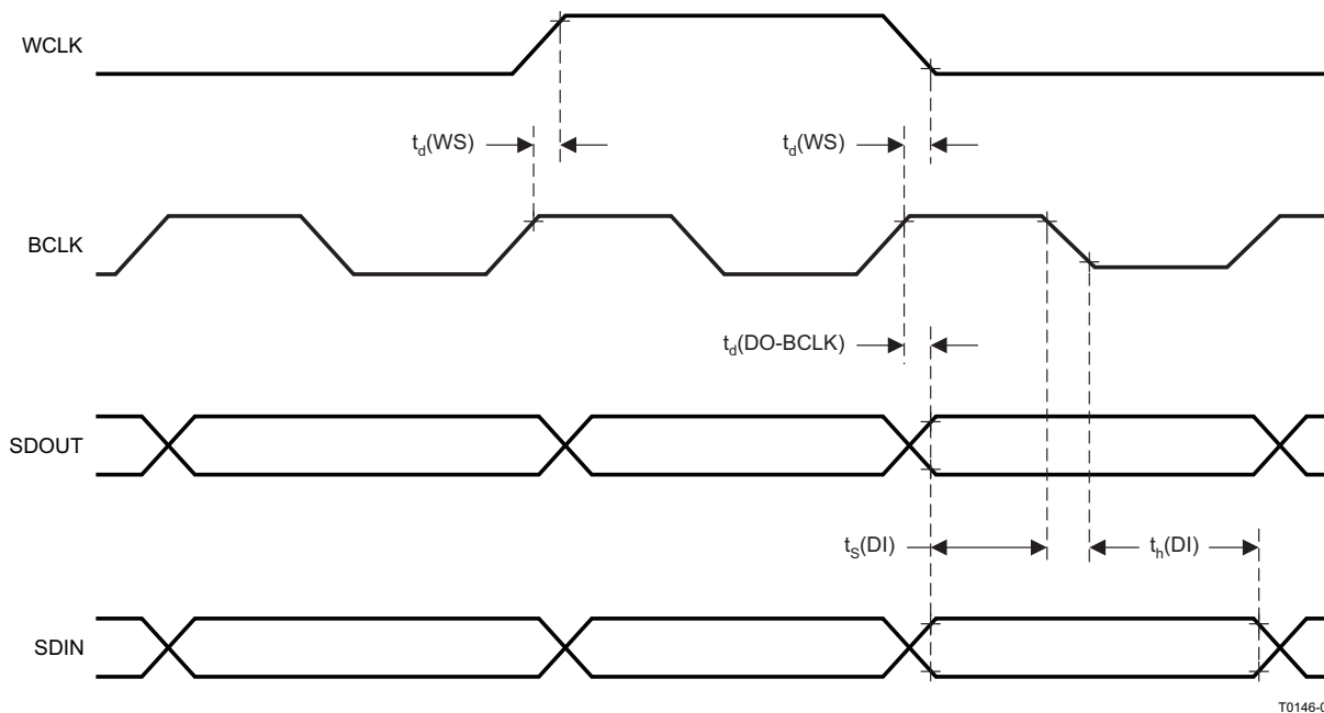
Figure 2. DSP Timing in Master Mode
