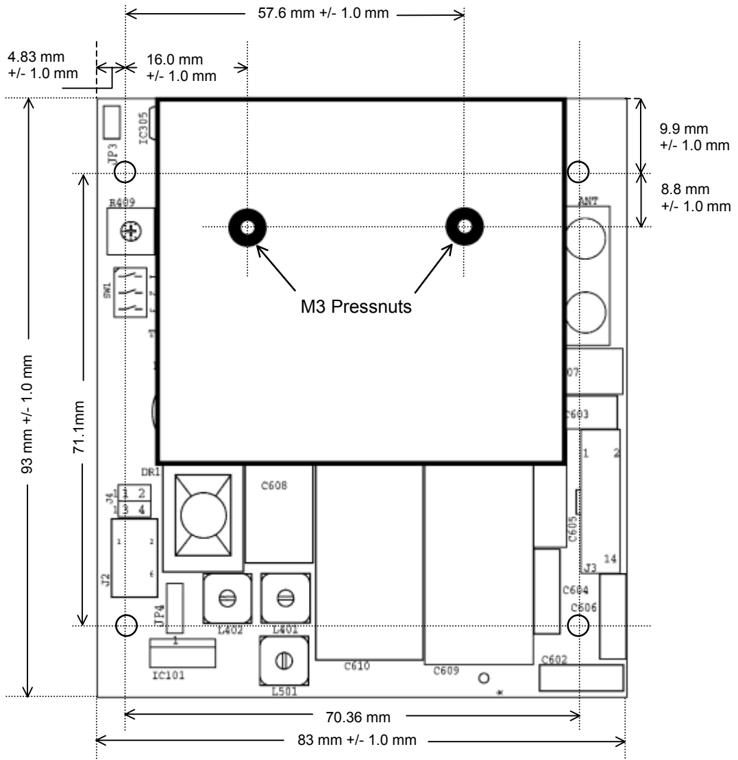
Figure 5: Mechanical Dimensions
