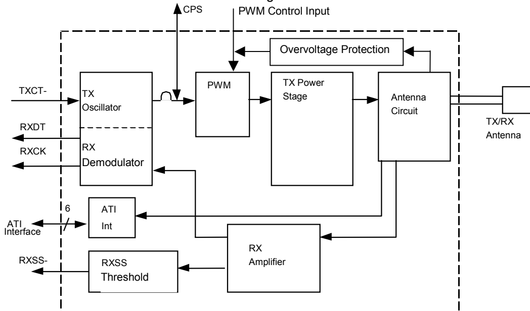
Figure 1: RFM Block Schematic
