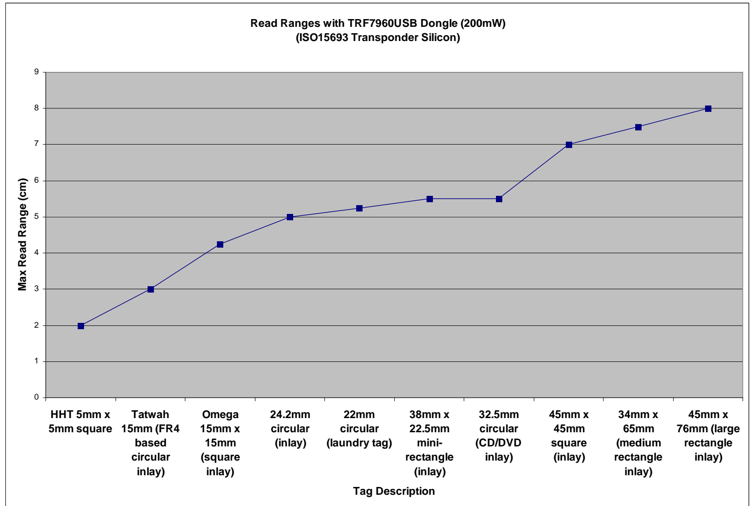
TRF7960USB Dongle
