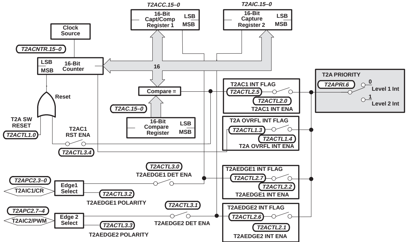
Figure 13. Dual-Capture Mode
