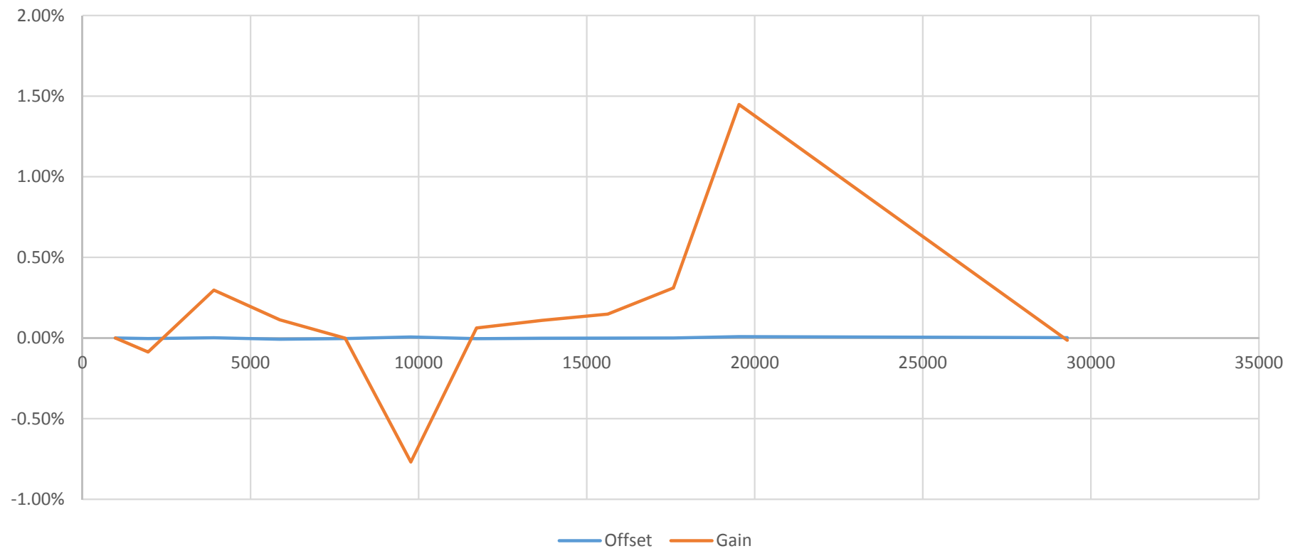
Error in ADS1278 vs Sampling Rate
