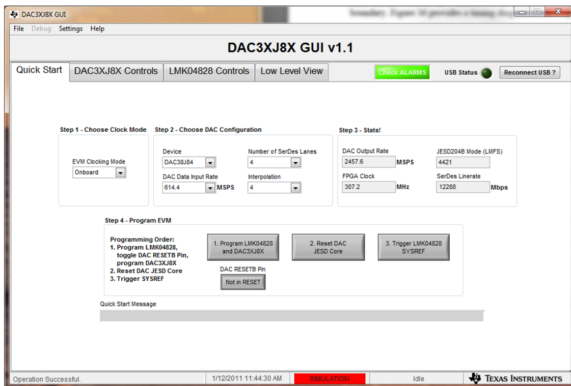
Figure 9. DAC38J84 Setting
