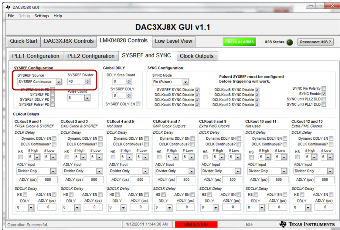
Figure 18. SYSREF Setting
