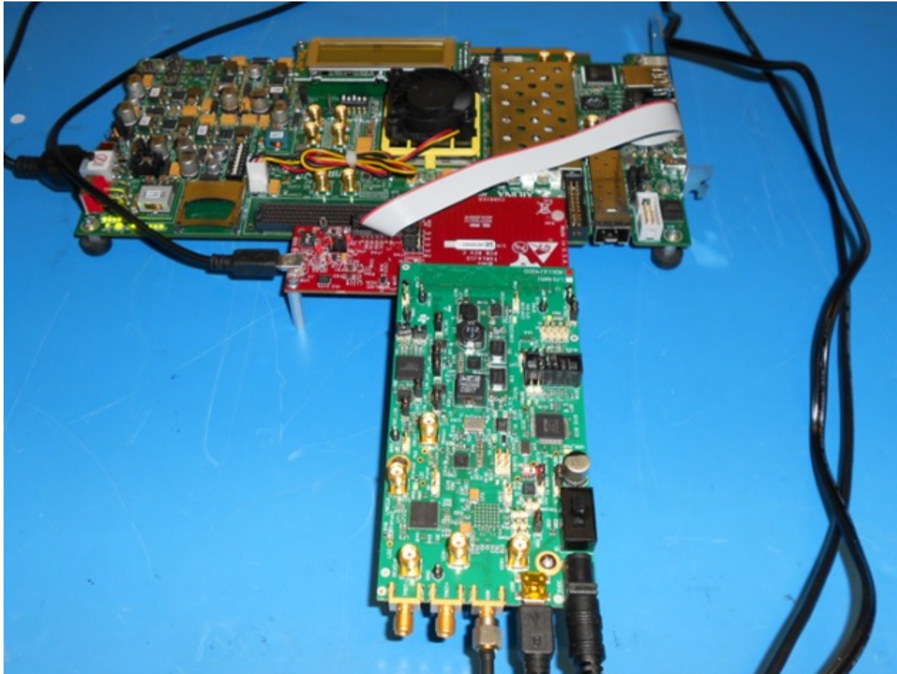
Figure 18. ADC12J4000EVM, TSW14J10EVM and VC707 Board
