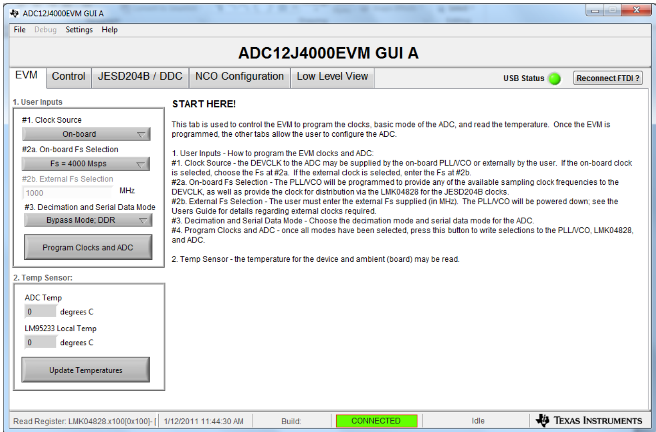
Figure 19. ADC12J4000EVM GUI
