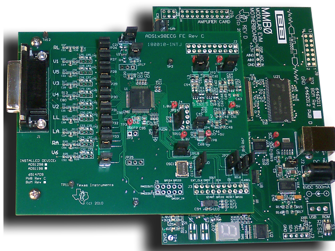
Figure 1. ADS1x98ECG-FE Kit
