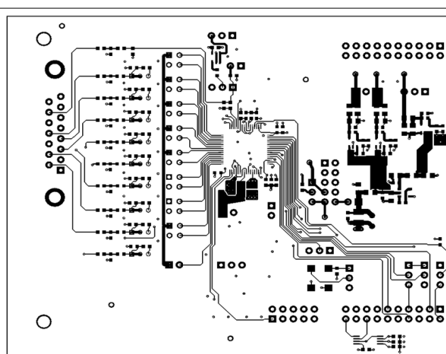
Figure 39. Top Layer
