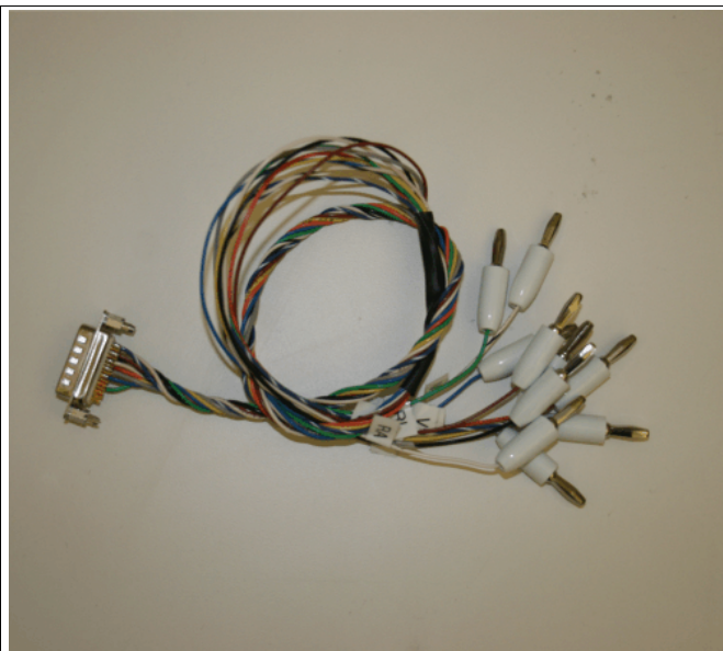
Figure 46. 15-Pin, Twisted Wire Cable to Banana Jacks
