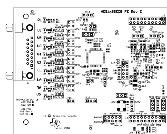
Figure 38. Top Component Placement
