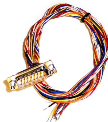
Figure 47. 15-Pin, Twisted Wire Cable
