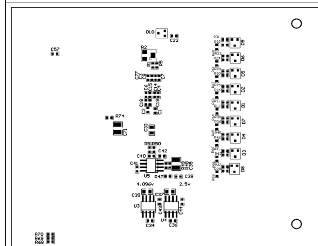
Figure 40. Bottom Component Placement
